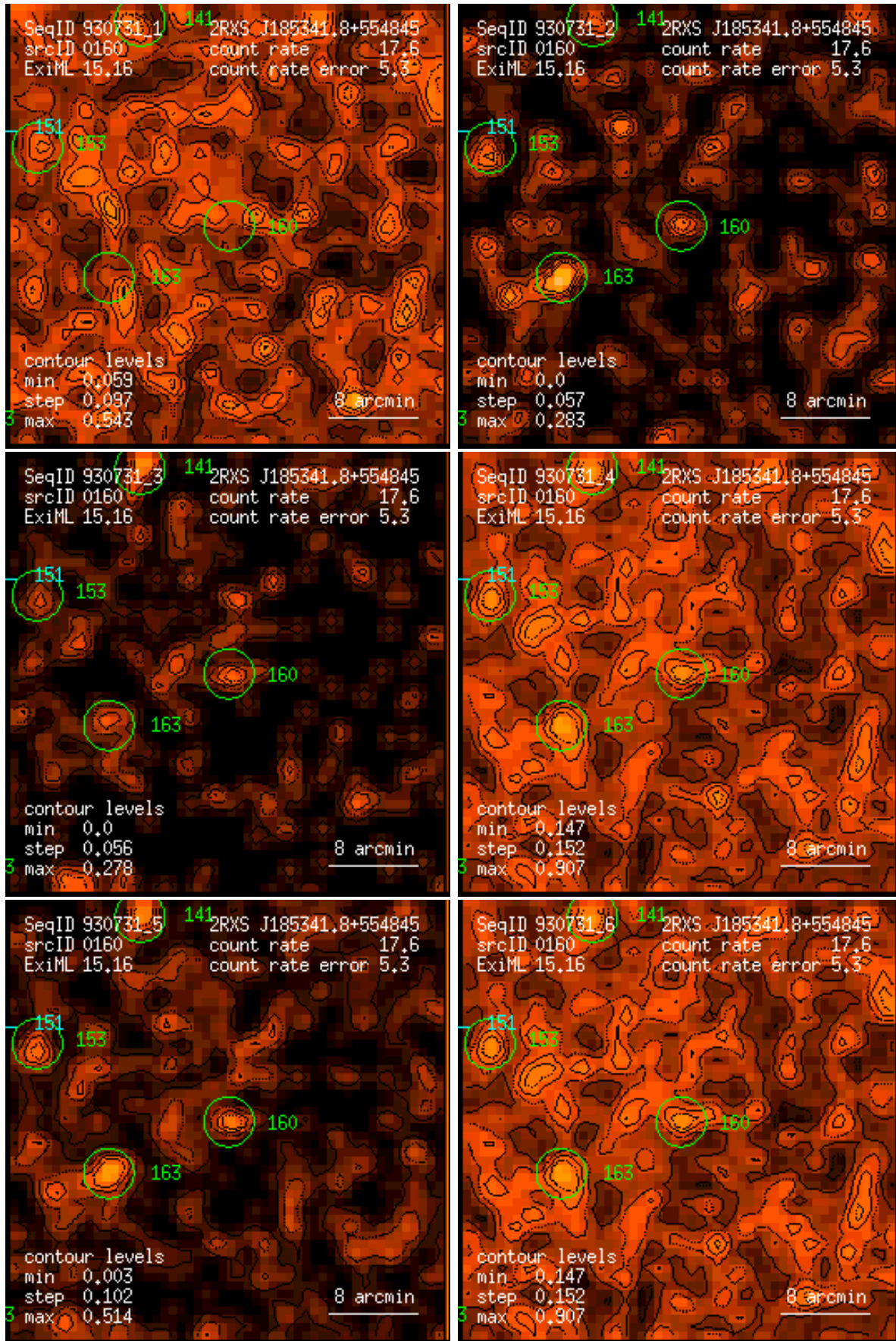
Figure 160: RASS 930731: detection 0160: band rate images, Gaussian filter: (1) PSPC channels 11 – 41, (2) 52 – 90, (3) 91 – 201, (4) 11 – 235, (5) 52 – 201, (6) 11 – 201. Broad band rates in counts/ks. Band rate contour levels in counts/ks/arcmin 2 .
