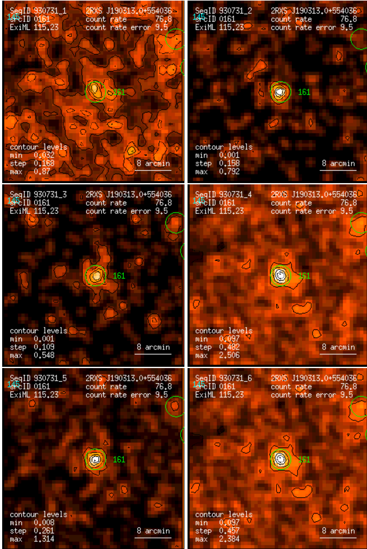
Figure 161: RASS 930731: detection 0161: band rate images, Gaussian filter: (1) PSPC channels 11 – 41, (2) 52 – 90, (3) 91 – 201, (4) 11 – 235, (5) 52 – 201, (6) 11 – 201. Broad band rates in counts/ks. Band rate contour levels in counts/ks/arcmin 2 .
