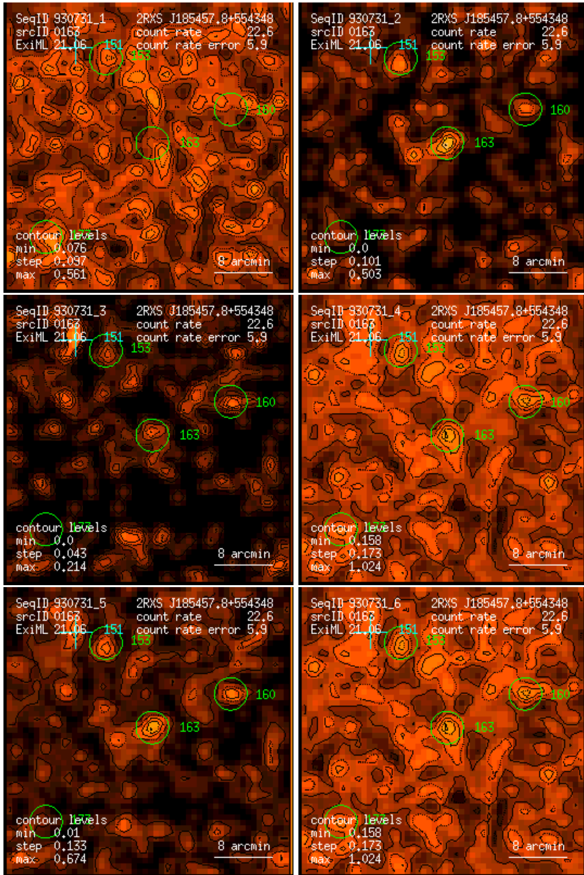
Figure 163: RASS 930731: detection 0163: band rate images, Gaussian filter: (1) PSPC channels 11 – 41, (2) 52 – 90, (3) 91 – 201, (4) 11 – 235, (5) 52 – 201, (6) 11 – 201. Broad band rates in counts/ks. Band rate contour levels in counts/ks/arcmin 2 .
