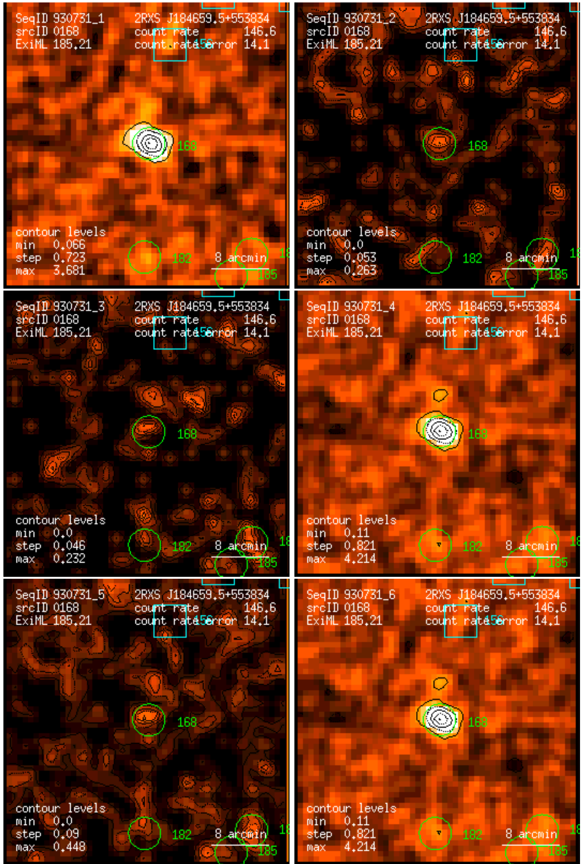
Figure 168: RASS 930731: detection 0168: band rate images, Gaussian filter: (1) PSPC channels 11 – 41, (2) 52 – 90, (3) 91 – 201, (4) 11 – 235, (5) 52 – 201, (6) 11 – 201. Broad band rates in counts/ks. Band rate contour levels in counts/ks/arcmin 2 .
