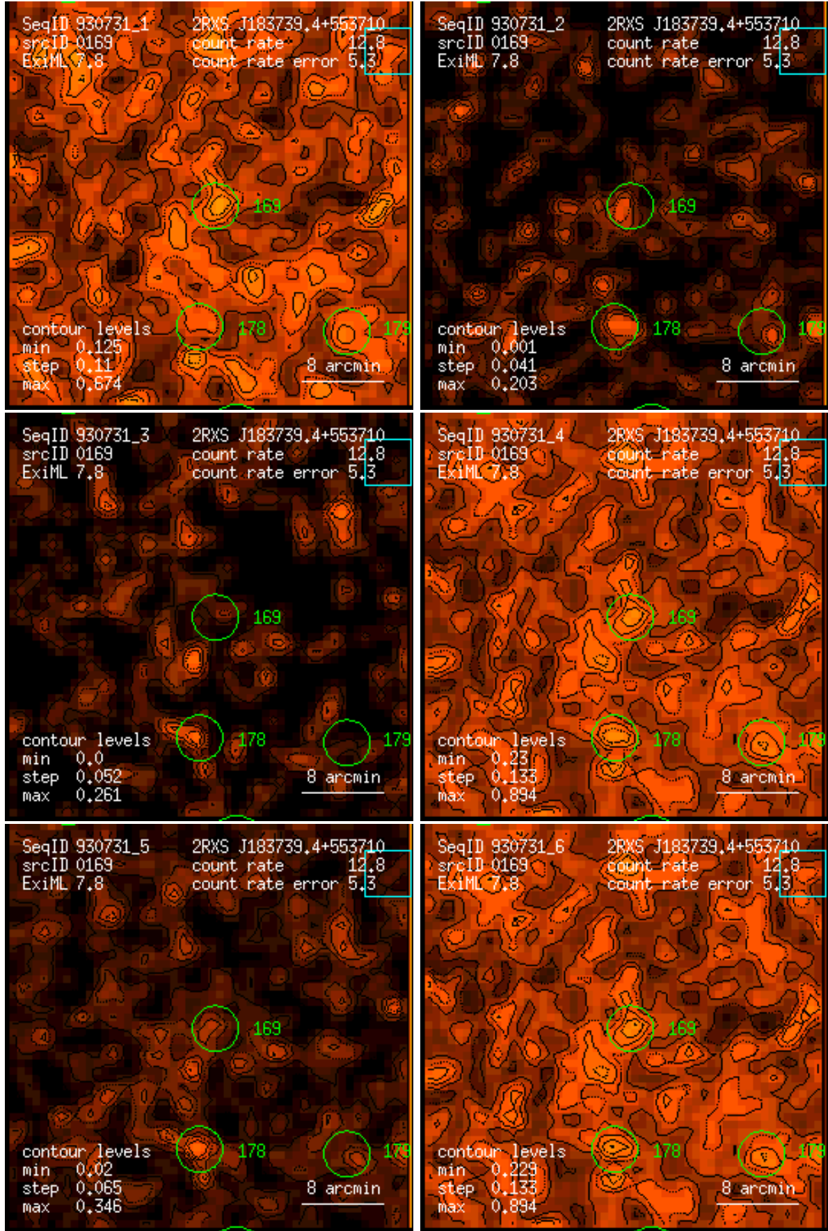
Figure 169: RASS 930731: detection 0169: band rate images, Gaussian filter: (1) PSPC channels 11 – 41, (2) 52 – 90, (3) 91 – 201, (4) 11 – 235, (5) 52 – 201, (6) 11 – 201. Broad band rates in counts/ks. Band rate contour levels in counts/ks/arcmin 2 .
