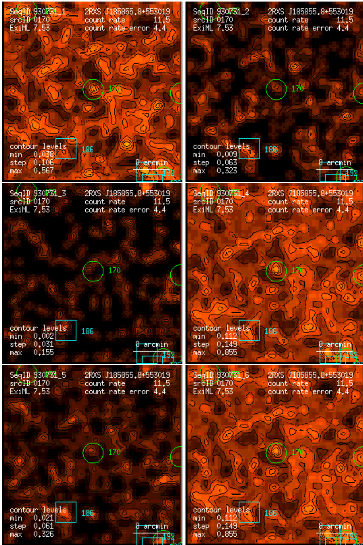
Figure 170: RASS 930731: detection 0170: band rate images, Gaussian filter: (1) PSPC channels 11 – 41, (2) 52 – 90, (3) 91 – 201, (4) 11 – 235, (5) 52 – 201, (6) 11 – 201. Broad band rates in counts/ks. Band rate contour levels in counts/ks/arcmin 2 .
