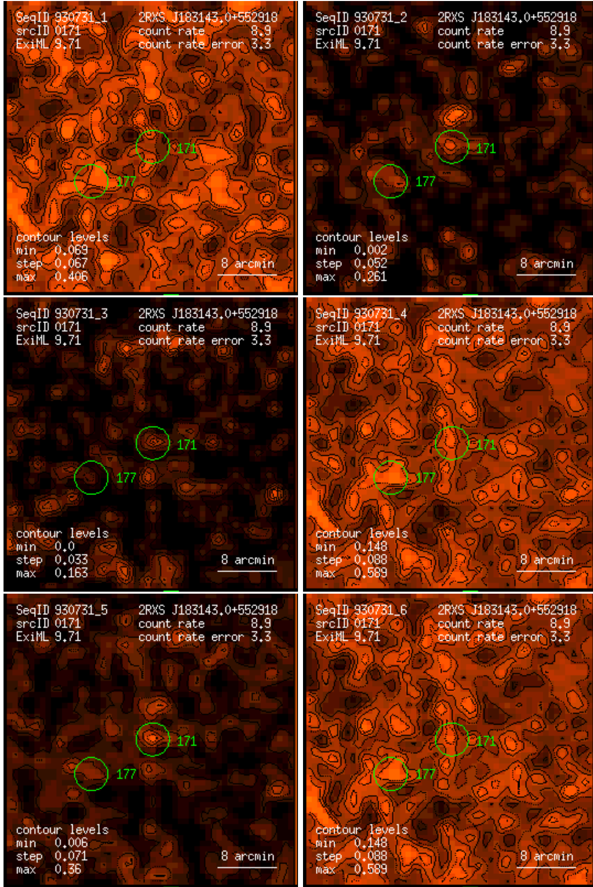
Figure 171: RASS 930731: detection 0171: band rate images, Gaussian filter: (1) PSPC channels 11 – 41, (2) 52 – 90, (3) 91 – 201, (4) 11 – 235, (5) 52 – 201, (6) 11 – 201. Broad band rates in counts/ks. Band rate contour levels in counts/ks/arcmin 2 .
