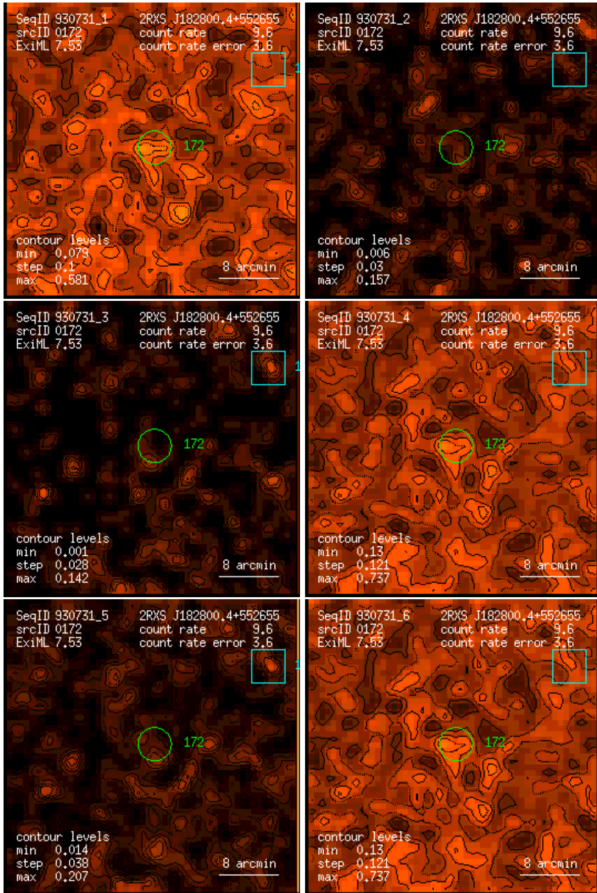
Figure 172: RASS 930731: detection 0172: band rate images, Gaussian filter: (1) PSPC channels 11 – 41, (2) 52 – 90, (3) 91 – 201, (4) 11 – 235, (5) 52 – 201, (6) 11 – 201. Broad band rates in counts/ks. Band rate contour levels in counts/ks/arcmin 2 .
