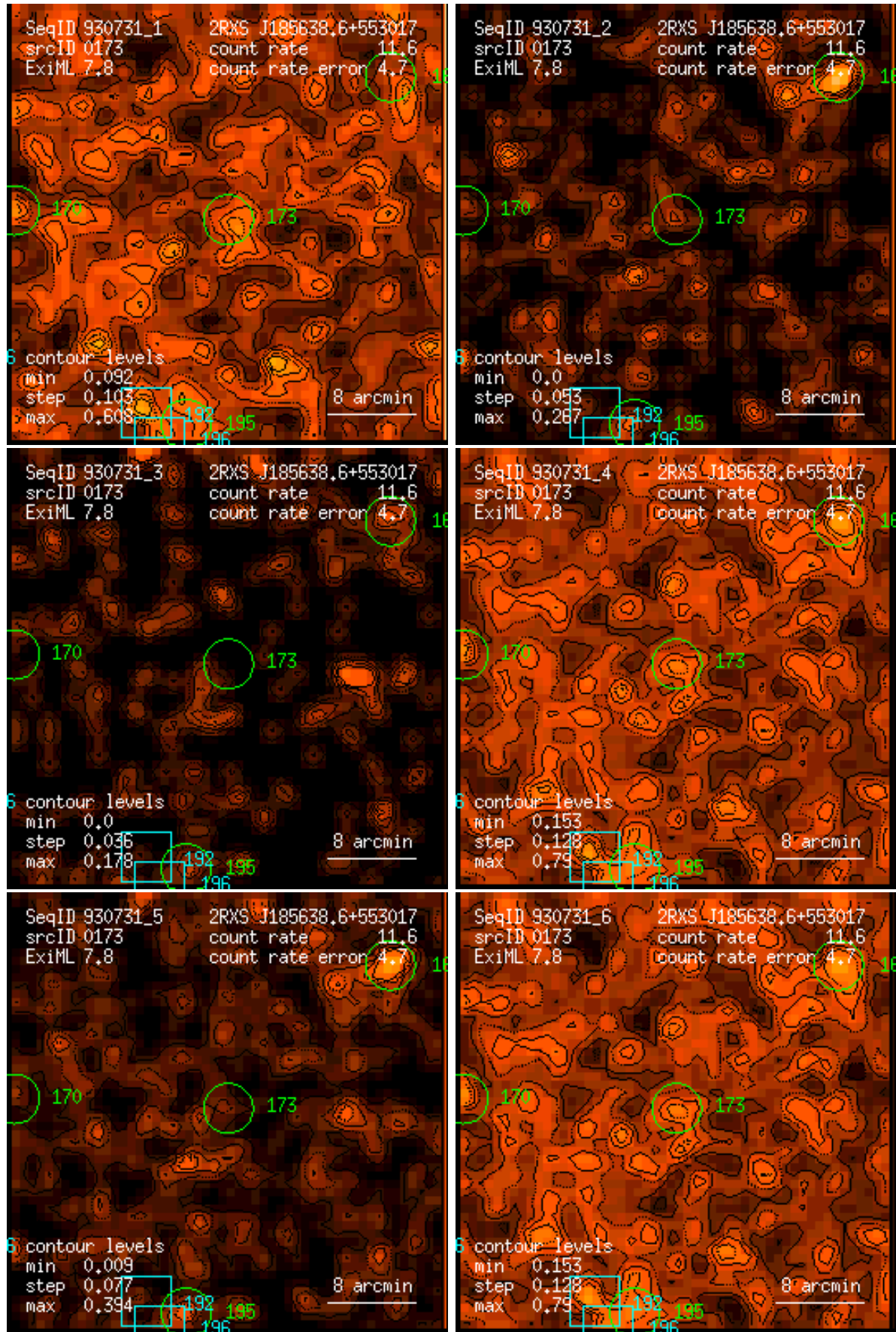
Figure 173: RASS 930731: detection 0173: band rate images, Gaussian filter: (1) PSPC channels 11 – 41, (2) 52 – 90, (3) 91 – 201, (4) 11 – 235, (5) 52 – 201, (6) 11 – 201. Broad band rates in counts/ks. Band rate contour levels in counts/ks/arcmin 2 .
