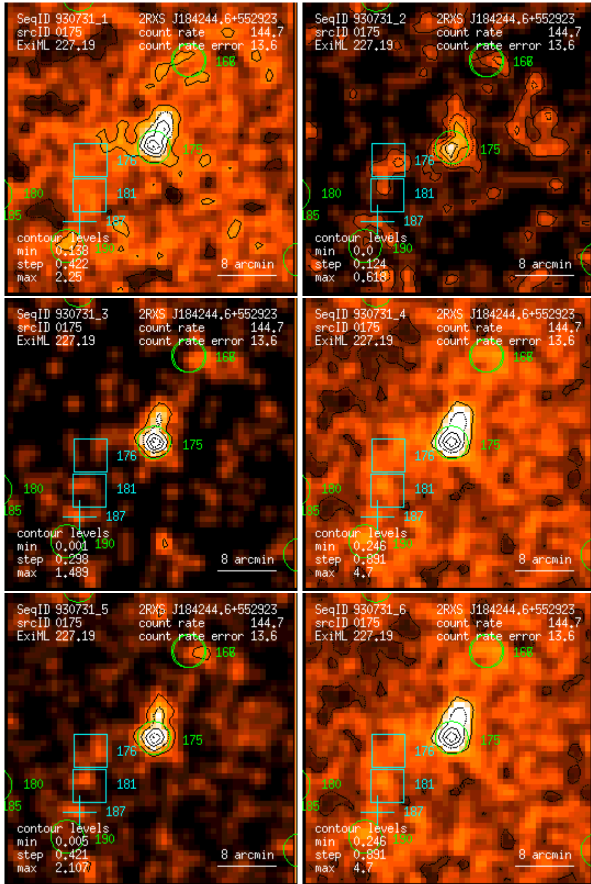
Figure 175: RASS 930731: detection 0175: band rate images, Gaussian filter: (1) PSPC channels 11 – 41, (2) 52 – 90, (3) 91 – 201, (4) 11 – 235, (5) 52 – 201, (6) 11 – 201. Broad band rates in counts/ks. Band rate contour levels in counts/ks/arcmin 2 .
