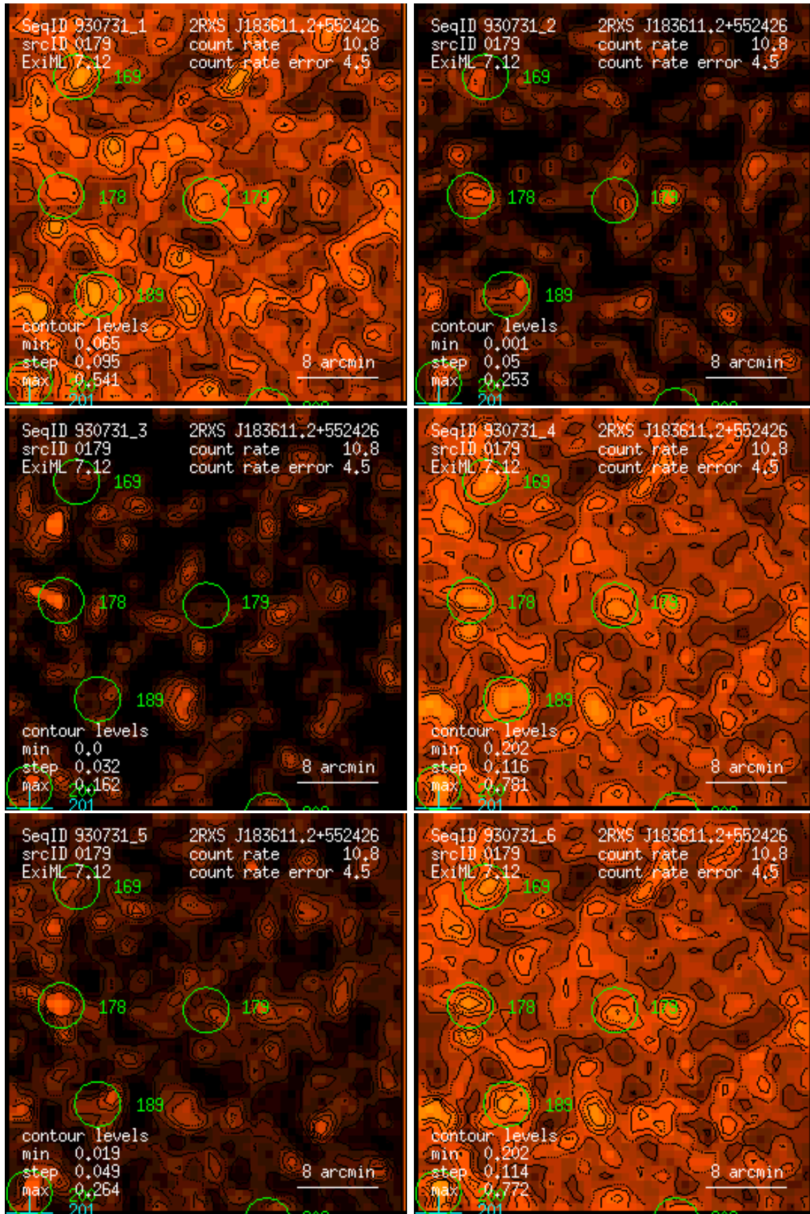
Figure 179: RASS 930731: detection 0179: band rate images, Gaussian filter: (1) PSPC channels 11 – 41, (2) 52 – 90, (3) 91 – 201, (4) 11 – 235, (5) 52 – 201, (6) 11 – 201. Broad band rates in counts/ks. Band rate contour levels in counts/ks/arcmin 2 .
