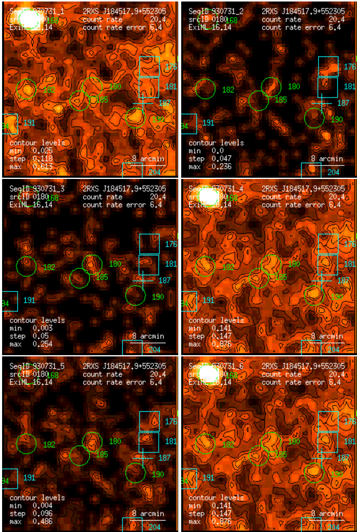
Figure 180: RASS 930731: detection 0180: band rate images, Gaussian filter: (1) PSPC channels 11 – 41, (2) 52 – 90, (3) 91 – 201, (4) 11 – 235, (5) 52 – 201, (6) 11 – 201. Broad band rates in counts/ks. Band rate contour levels in counts/ks/arcmin 2 .
