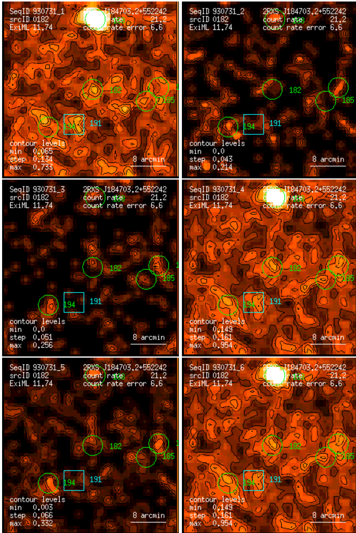
Figure 182: RASS 930731: detection 0182: band rate images, Gaussian filter: (1) PSPC channels 11 – 41, (2) 52 – 90, (3) 91 – 201, (4) 11 – 235, (5) 52 – 201, (6) 11 – 201. Broad band rates in counts/ks. Band rate contour levels in counts/ks/arcmin 2 .
