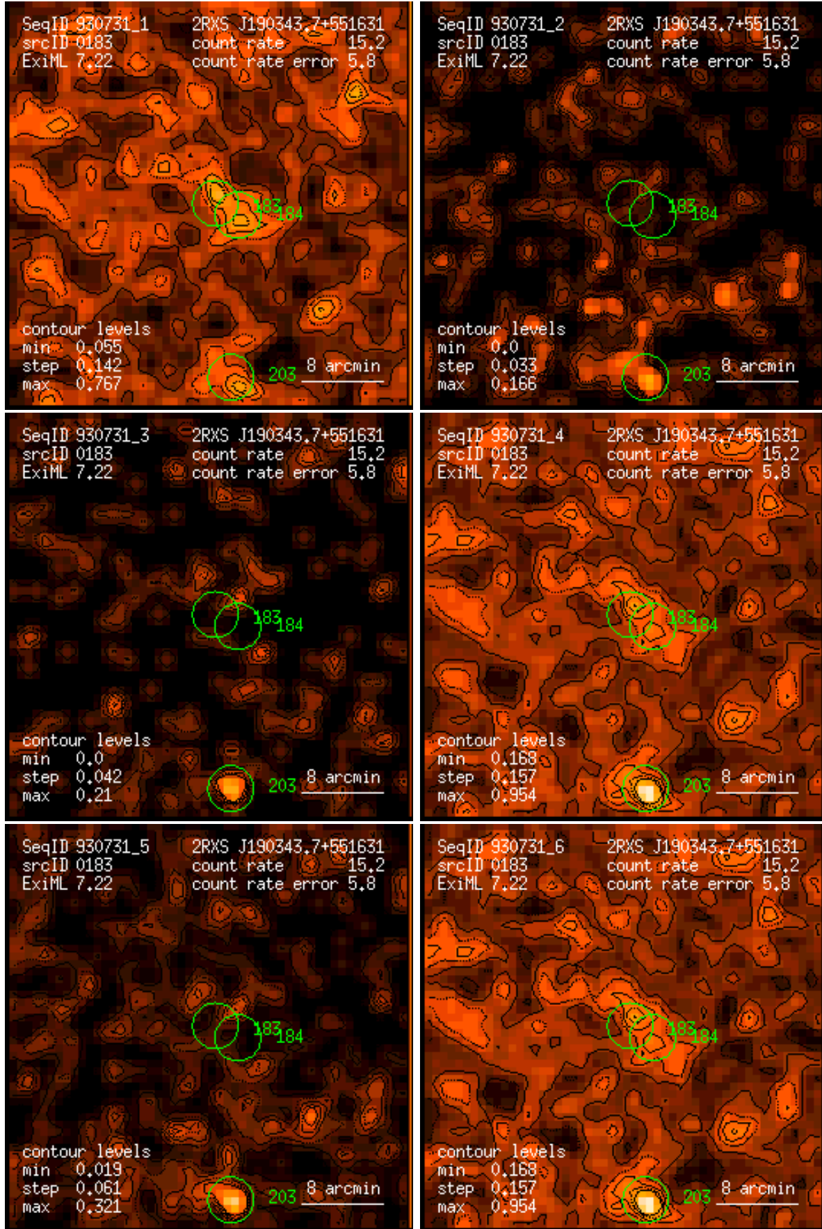
Figure 183: RASS 930731: detection 0183: band rate images, Gaussian filter: (1) PSPC channels 11 – 41, (2) 52 – 90, (3) 91 – 201, (4) 11 – 235, (5) 52 – 201, (6) 11 – 201. Broad band rates in counts/ks. Band rate contour levels in counts/ks/arcmin 2 .
