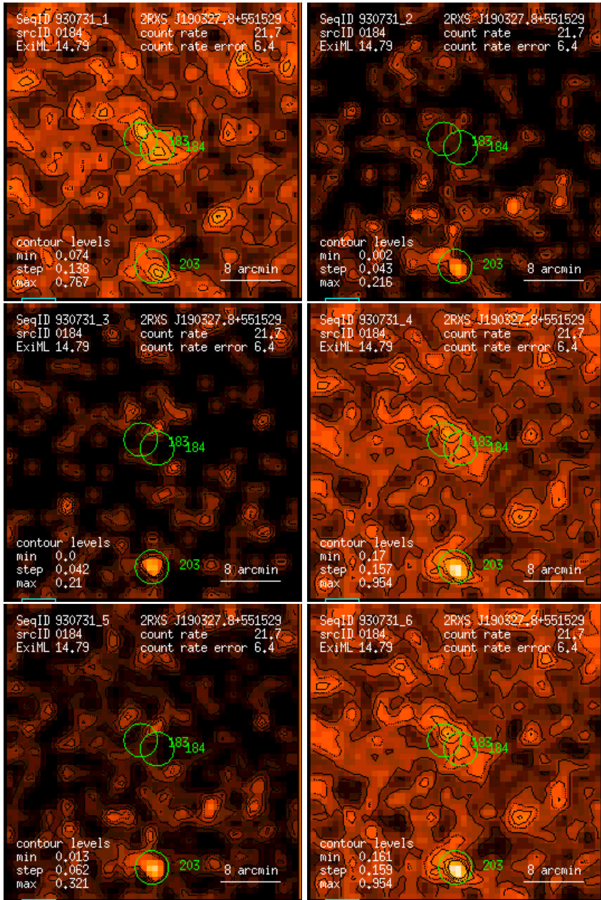
Figure 184: RASS 930731: detection 0184: band rate images, Gaussian filter: (1) PSPC channels 11 – 41, (2) 52 – 90, (3) 91 – 201, (4) 11 – 235, (5) 52 – 201, (6) 11 – 201. Broad band rates in counts/ks. Band rate contour levels in counts/ks/arcmin 2 .
