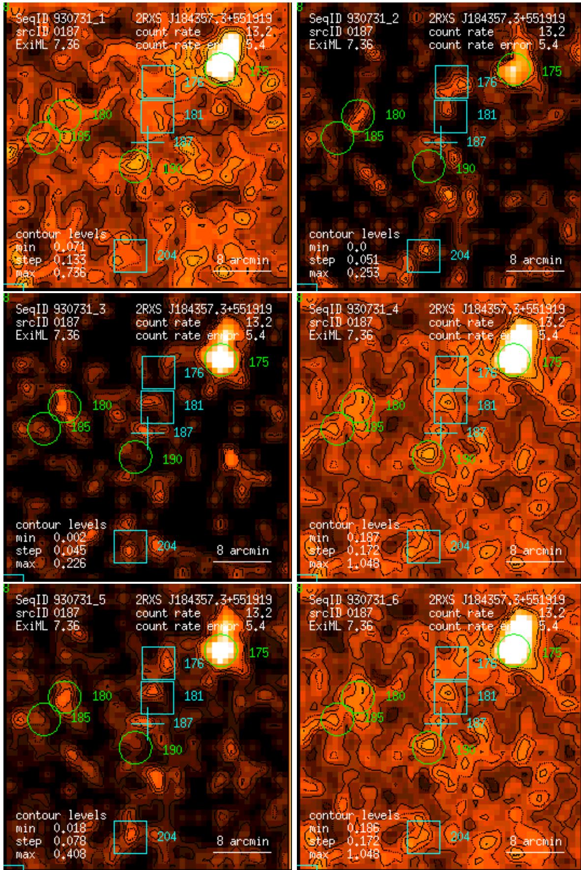
Figure 187: RASS 930731: detection 0187: band rate images, Gaussian filter: (1) PSPC channels 11 – 41, (2) 52 – 90, (3) 91 – 201, (4) 11 – 235, (5) 52 – 201, (6) 11 – 201. Broad band rates in counts/ks. Band rate contour levels in counts/ks/arcmin 2 .
