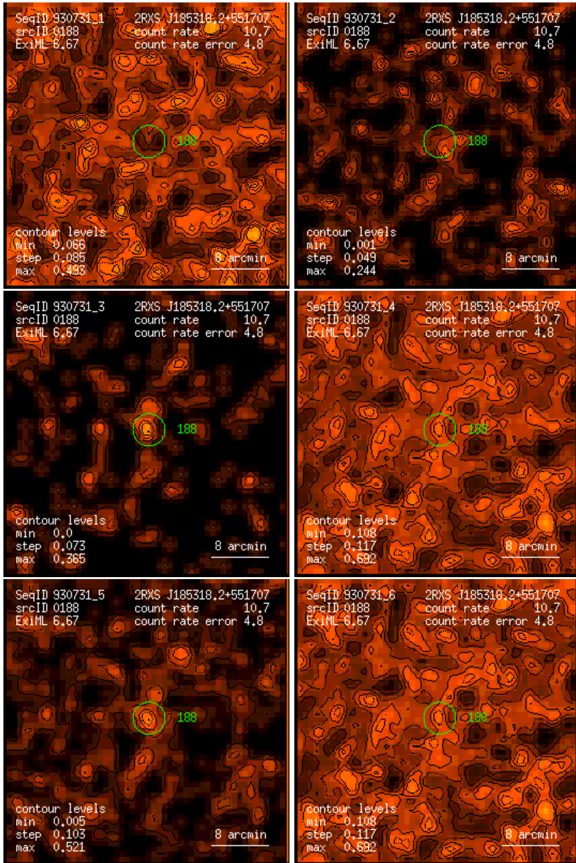
Figure 188: RASS 930731: detection 0188: band rate images, Gaussian filter: (1) PSPC channels 11 – 41, (2) 52 – 90, (3) 91 – 201, (4) 11 – 235, (5) 52 – 201, (6) 11 – 201. Broad band rates in counts/ks. Band rate contour levels in counts/ks/arcmin 2 .
