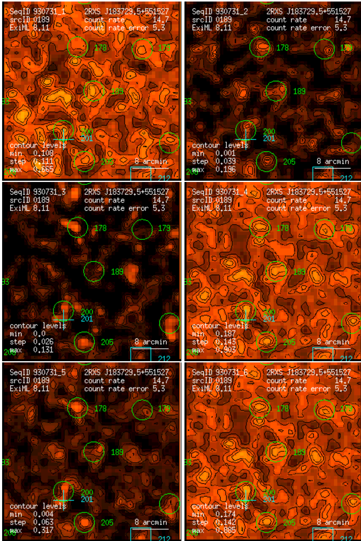
Figure 189: RASS 930731: detection 0189: band rate images, Gaussian filter: (1) PSPC channels 11 – 41, (2) 52 – 90, (3) 91 – 201, (4) 11 – 235, (5) 52 – 201, (6) 11 – 201. Broad band rates in counts/ks. Band rate contour levels in counts/ks/arcmin 2 .
