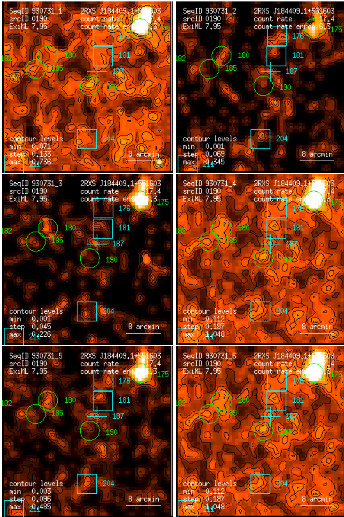
Figure 190: RASS 930731: detection 0190: band rate images, Gaussian filter: (1) PSPC channels 11 – 41, (2) 52 – 90, (3) 91 – 201, (4) 11 – 235, (5) 52 – 201, (6) 11 – 201. Broad band rates in counts/ks. Band rate contour levels in counts/ks/arcmin 2 .
