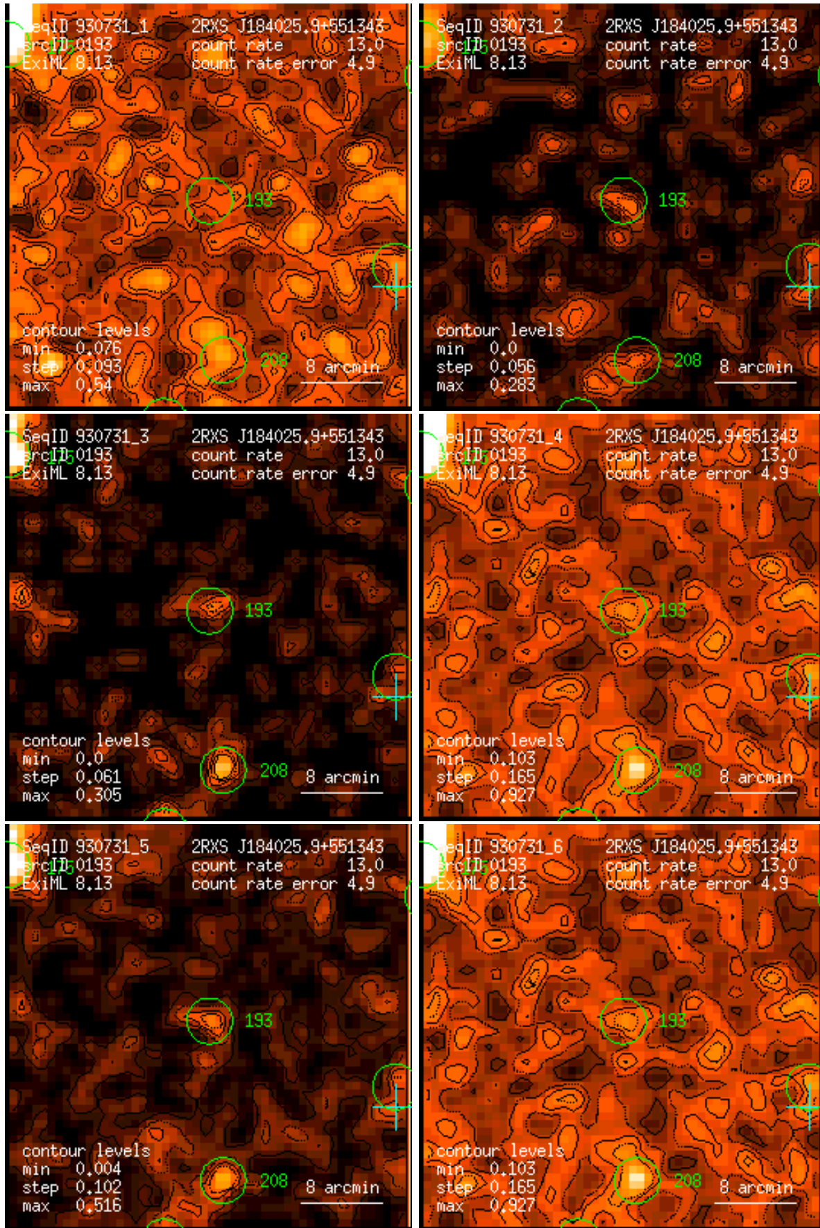
Figure 193: RASS 930731: detection 0193: band rate images, Gaussian filter: (1) PSPC channels 11 – 41, (2) 52 – 90, (3) 91 – 201, (4) 11 – 235, (5) 52 – 201, (6) 11 – 201. Broad band rates in counts/ks. Band rate contour levels in counts/ks/arcmin 2 .
