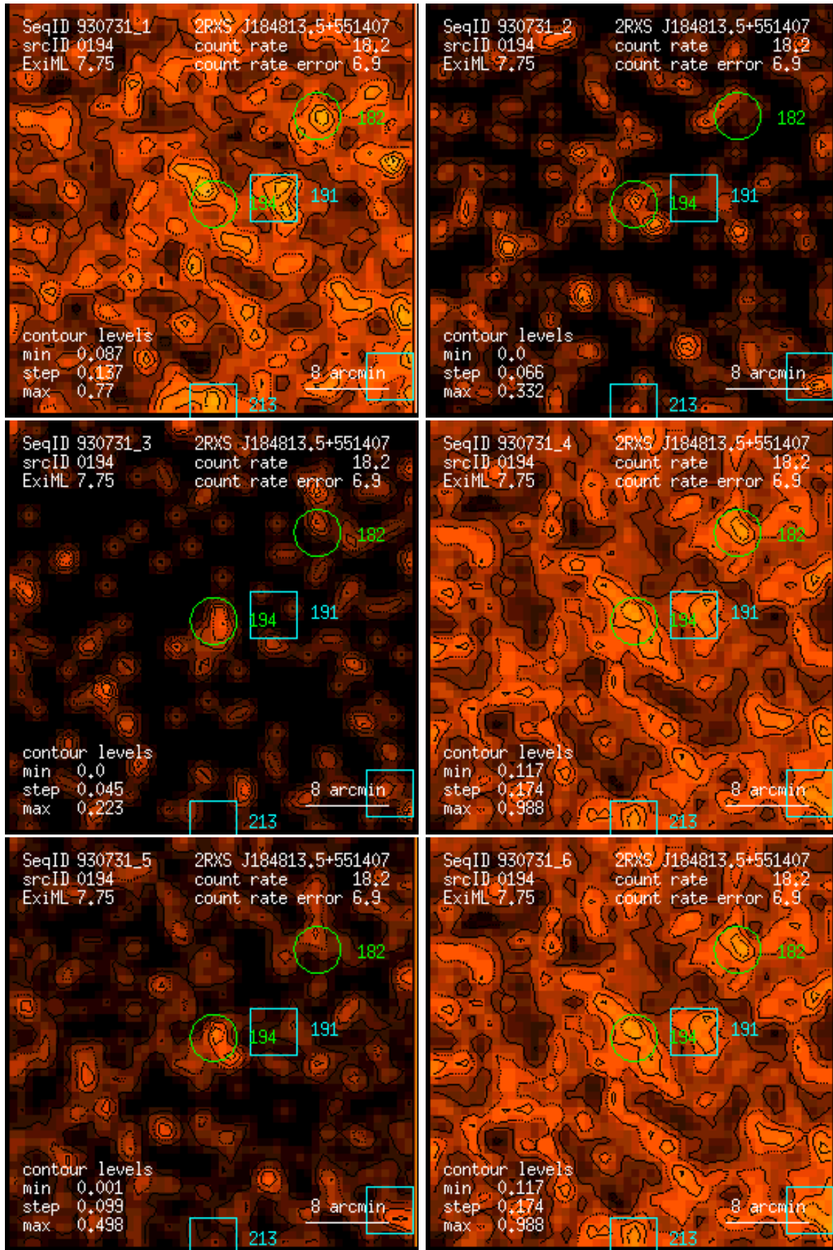
Figure 194: RASS 930731: detection 0194: band rate images, Gaussian filter: (1) PSPC channels 11 – 41, (2) 52 – 90, (3) 91 – 201, (4) 11 – 235, (5) 52 – 201, (6) 11 – 201. Broad band rates in counts/ks. Band rate contour levels in counts/ks/arcmin 2 .
