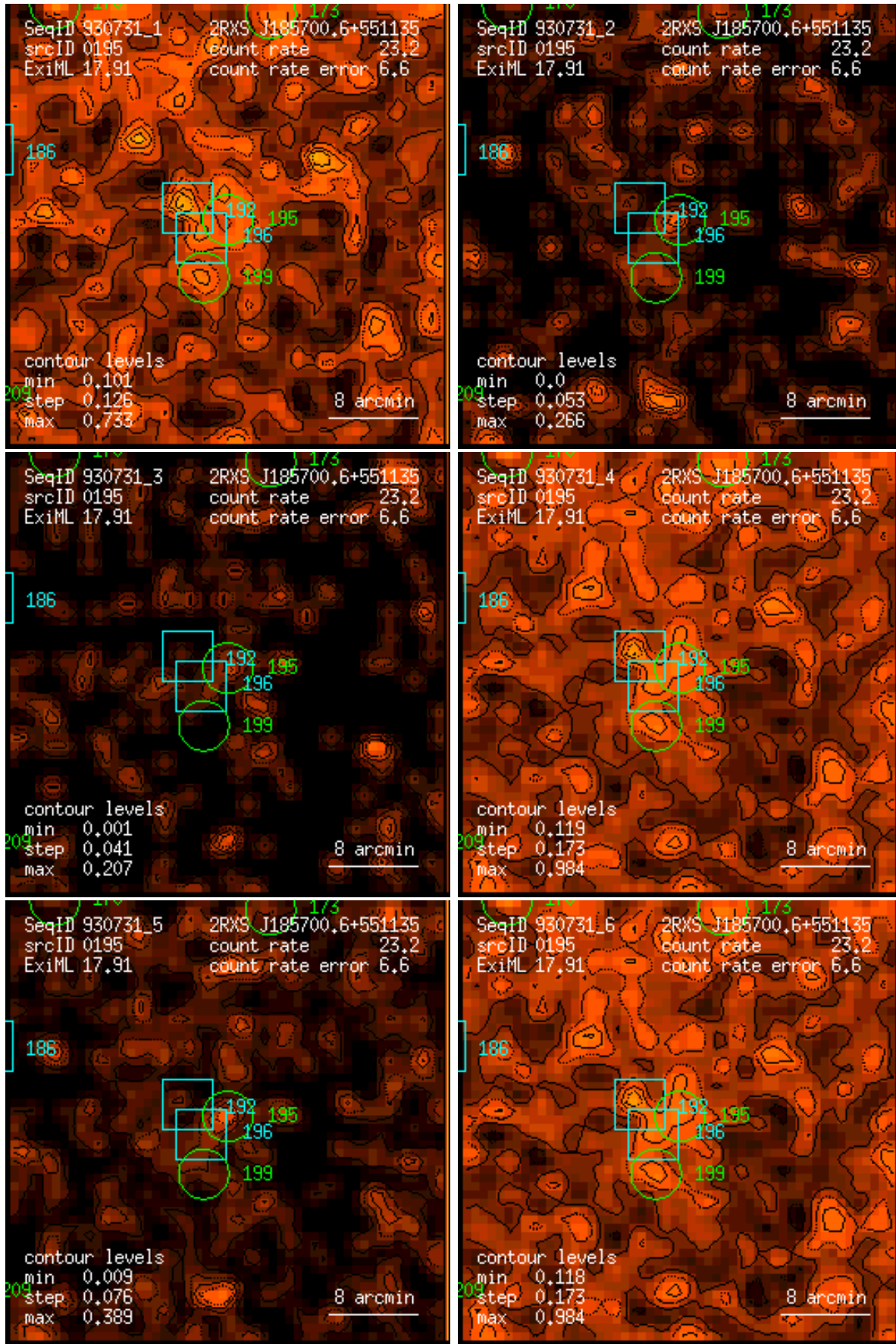
Figure 195: RASS 930731: detection 0195: band rate images, Gaussian filter: (1) PSPC channels 11 – 41, (2) 52 – 90, (3) 91 – 201, (4) 11 – 235, (5) 52 – 201, (6) 11 – 201. Broad band rates in counts/ks. Band rate contour levels in counts/ks/arcmin 2 .
