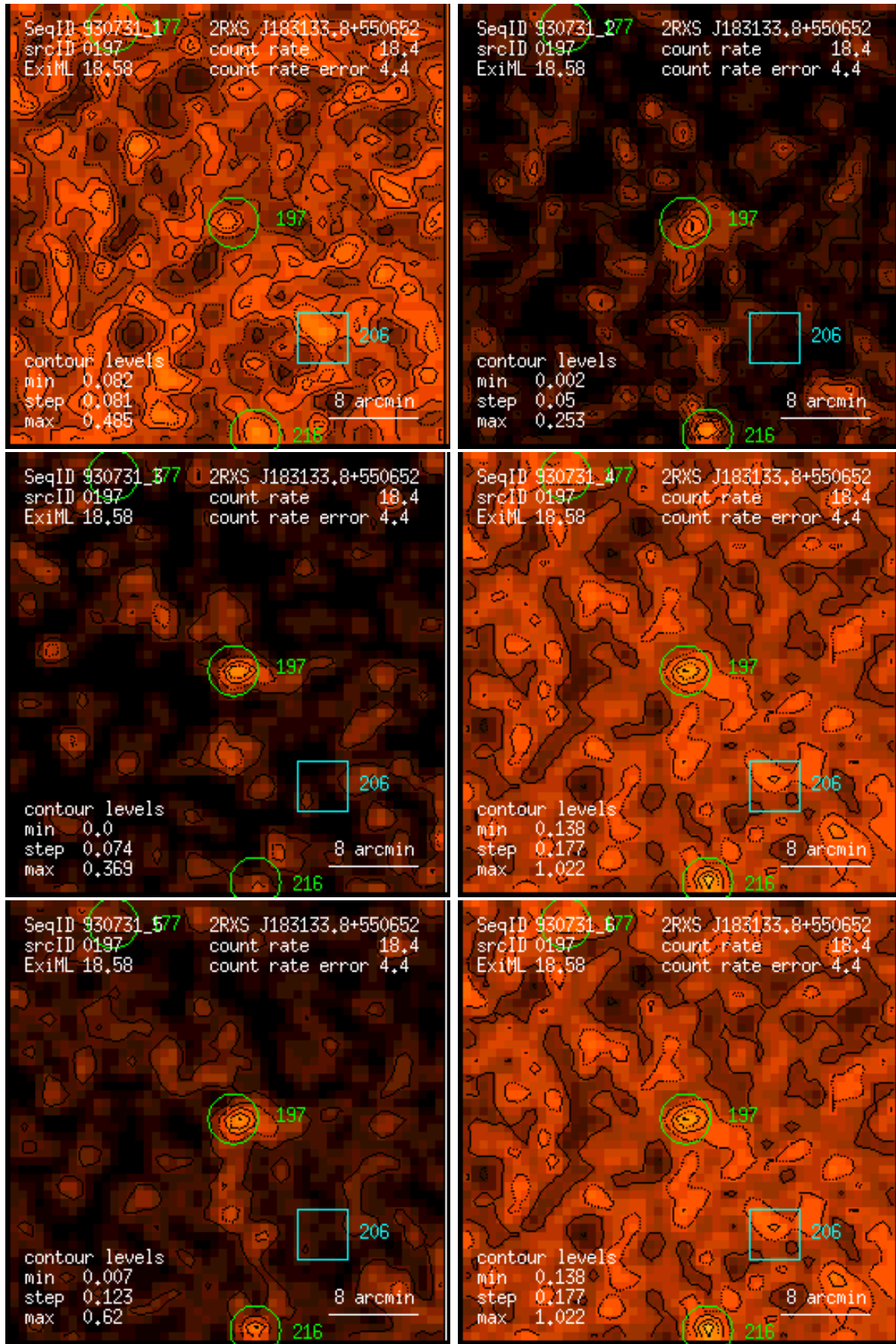
Figure 197: RASS 930731: detection 0197: band rate images, Gaussian filter: (1) PSPC channels 11 – 41, (2) 52 – 90, (3) 91 – 201, (4) 11 – 235, (5) 52 – 201, (6) 11 – 201. Broad band rates in counts/ks. Band rate contour levels in counts/ks/arcmin 2 .
