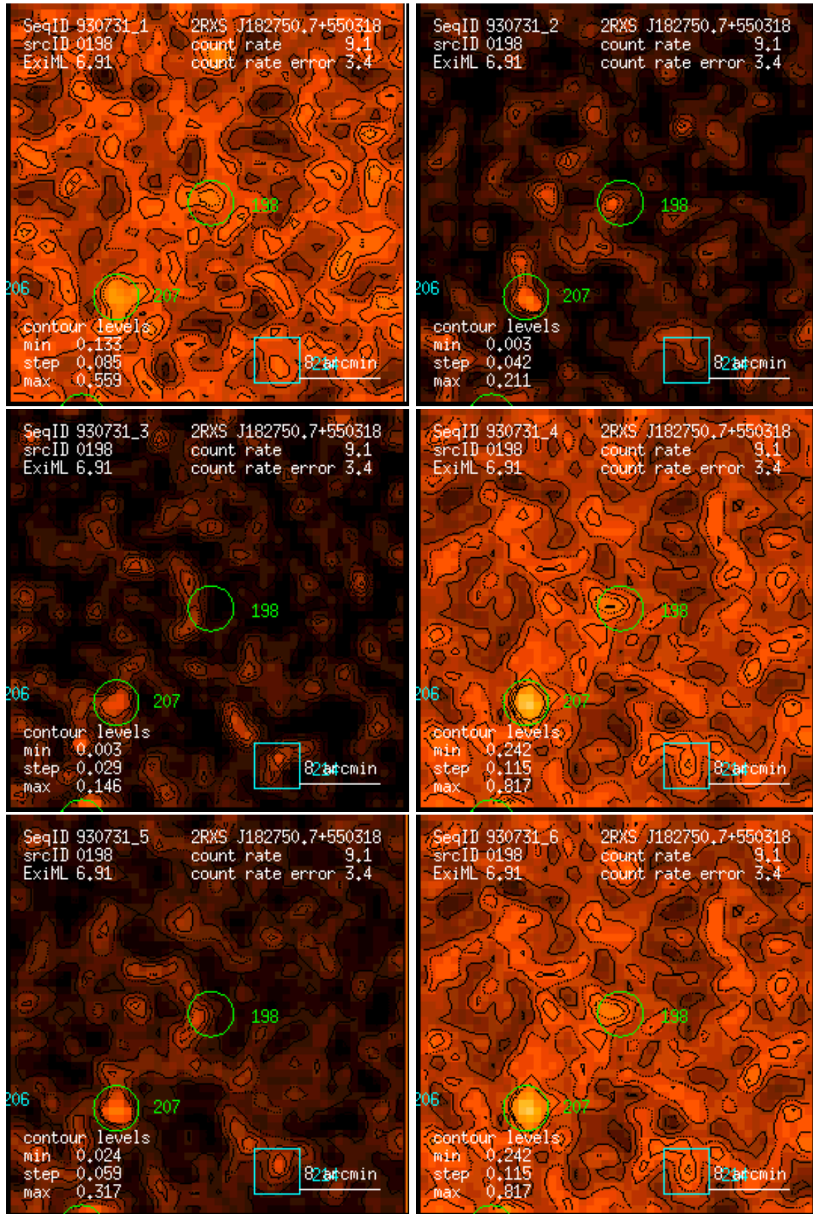
Figure 198: RASS 930731: detection 0198: band rate images, Gaussian filter: (1) PSPC channels 11 – 41, (2) 52 – 90, (3) 91 – 201, (4) 11 – 235, (5) 52 – 201, (6) 11 – 201. Broad band rates in counts/ks. Band rate contour levels in counts/ks/arcmin 2 .
