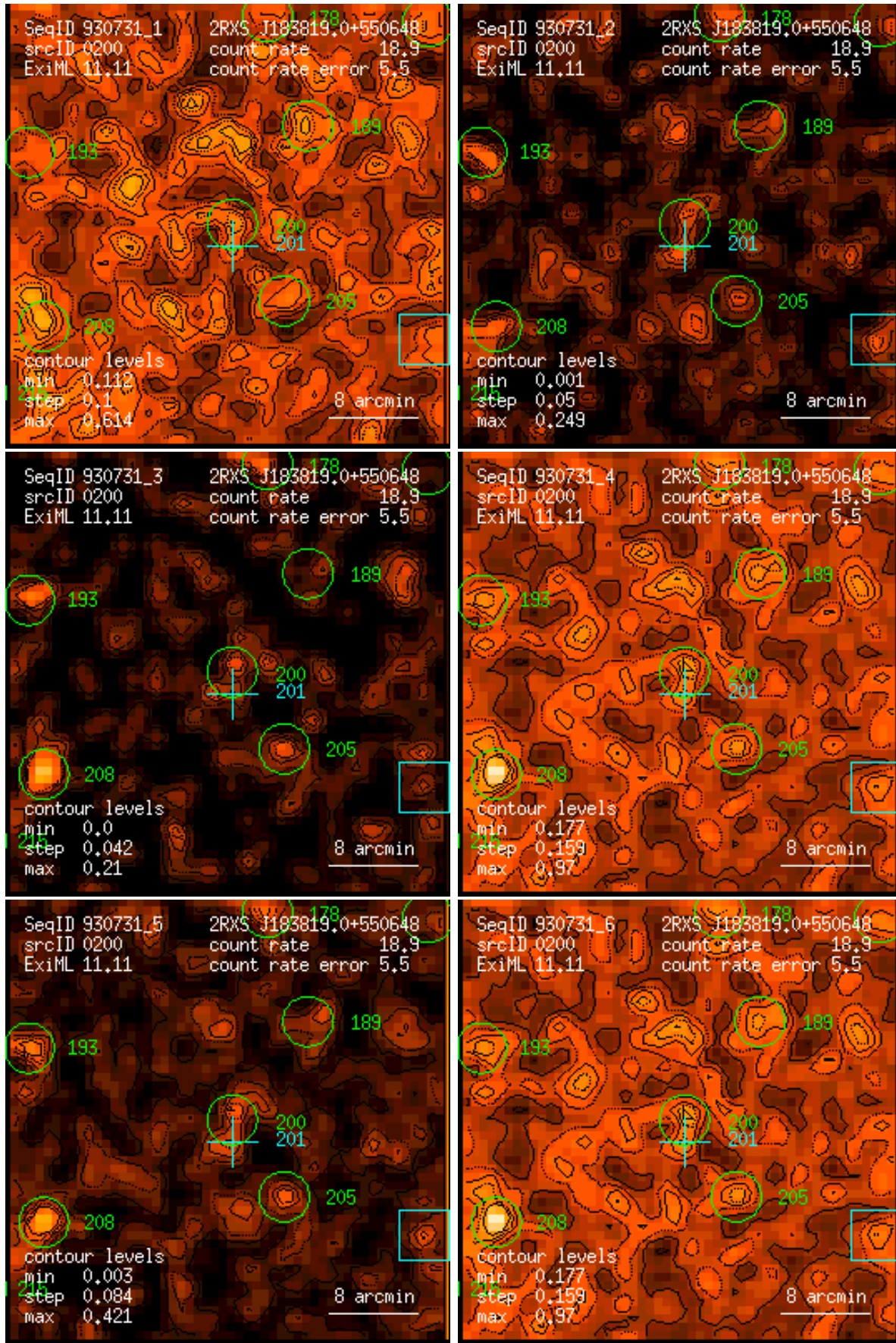
Figure 200: RASS 930731: detection 0200: band rate images, Gaussian filter: (1) PSPC channels 11 – 41, (2) 52 – 90, (3) 91 – 201, (4) 11 – 235, (5) 52 – 201, (6) 11 – 201. Broad band rates in counts/ks. Band rate contour levels in counts/ks/arcmin 2 .
