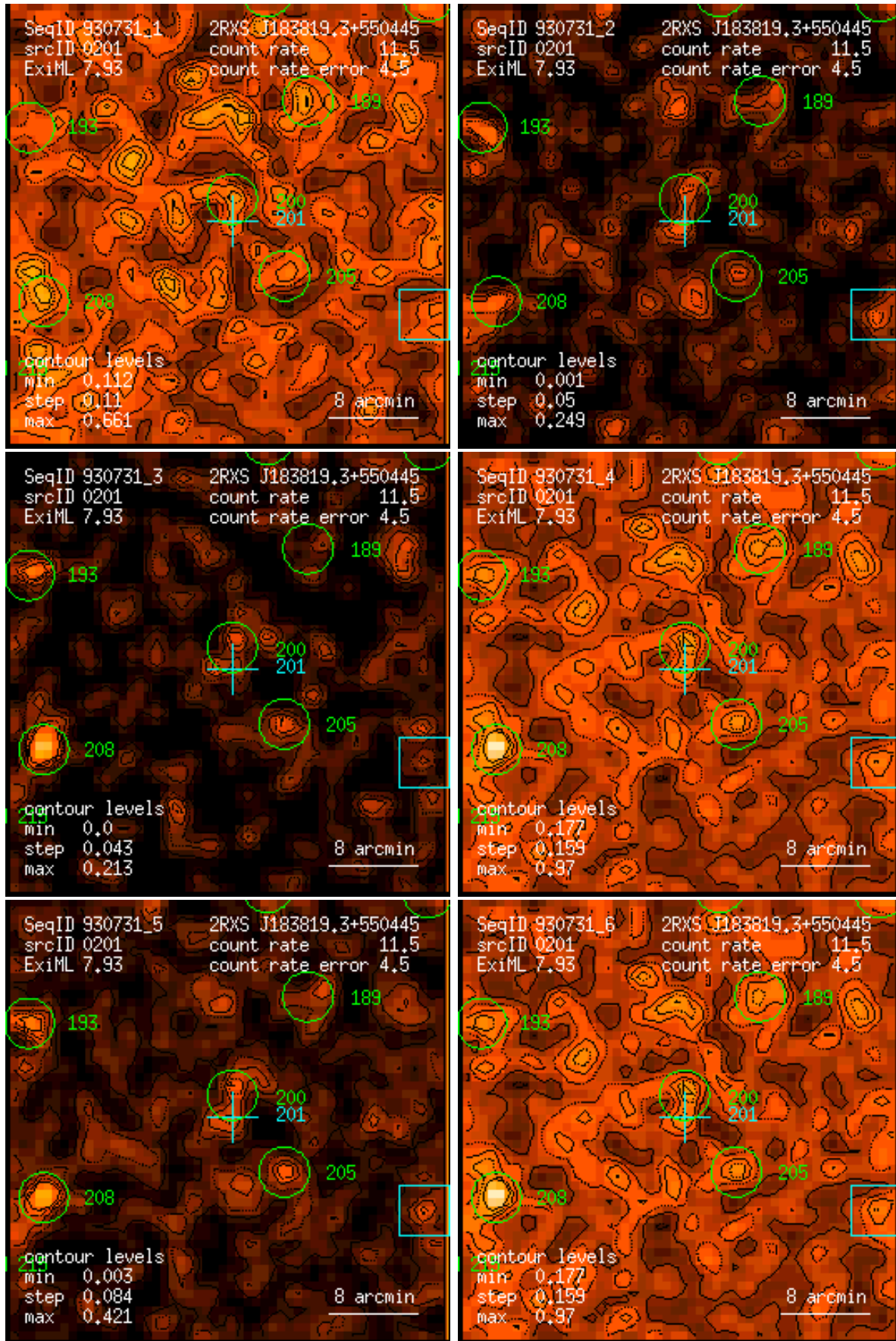
Figure 201: RASS 930731: detection 0201: band rate images, Gaussian filter: (1) PSPC channels 11 – 41, (2) 52 – 90, (3) 91 – 201, (4) 11 – 235, (5) 52 – 201, (6) 11 – 201. Broad band rates in counts/ks. Band rate contour levels in counts/ks/arcmin 2 .
