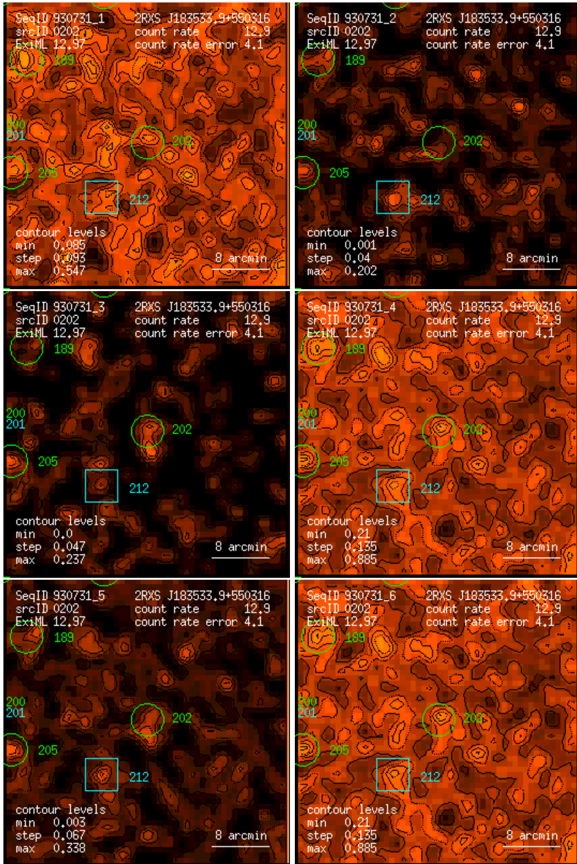
Figure 202: RASS 930731: detection 0202: band rate images, Gaussian filter: (1) PSPC channels 11 – 41, (2) 52 – 90, (3) 91 – 201, (4) 11 – 235, (5) 52 – 201, (6) 11 – 201. Broad band rates in counts/ks. Band rate contour levels in counts/ks/arcmin 2 .
