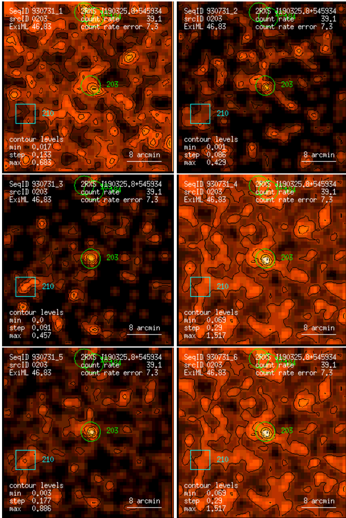
Figure 203: RASS 930731: detection 0203: band rate images, Gaussian filter: (1) PSPC channels 11 – 41, (2) 52 – 90, (3) 91 – 201, (4) 11 – 235, (5) 52 – 201, (6) 11 – 201. Broad band rates in counts/ks. Band rate contour levels in counts/ks/arcmin 2 .
