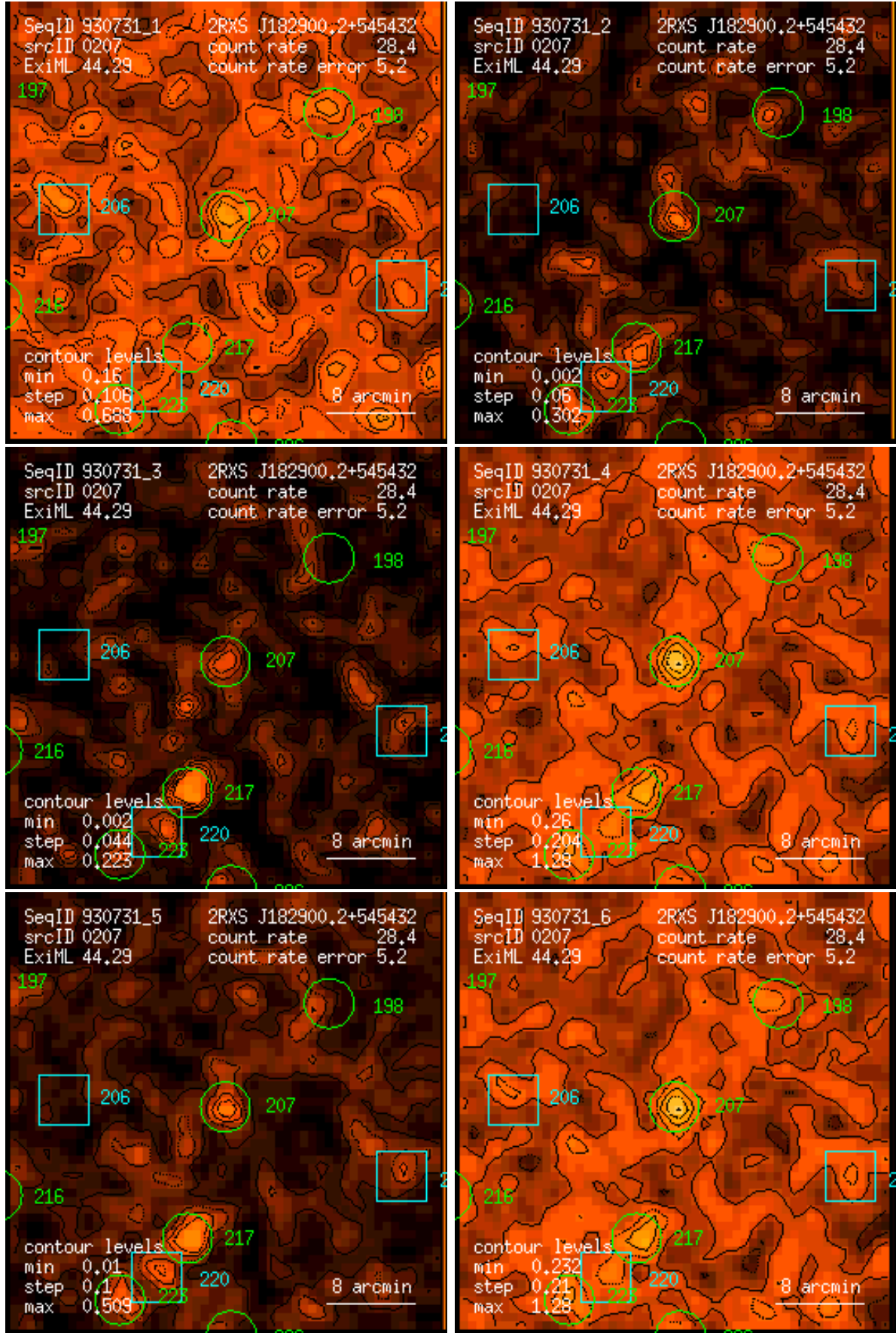
Figure 207: RASS 930731: detection 0207: band rate images, Gaussian filter: (1) PSPC channels 11 – 41, (2) 52 – 90, (3) 91 – 201, (4) 11 – 235, (5) 52 – 201, (6) 11 – 201. Broad band rates in counts/ks. Band rate contour levels in counts/ks/arcmin 2 .
