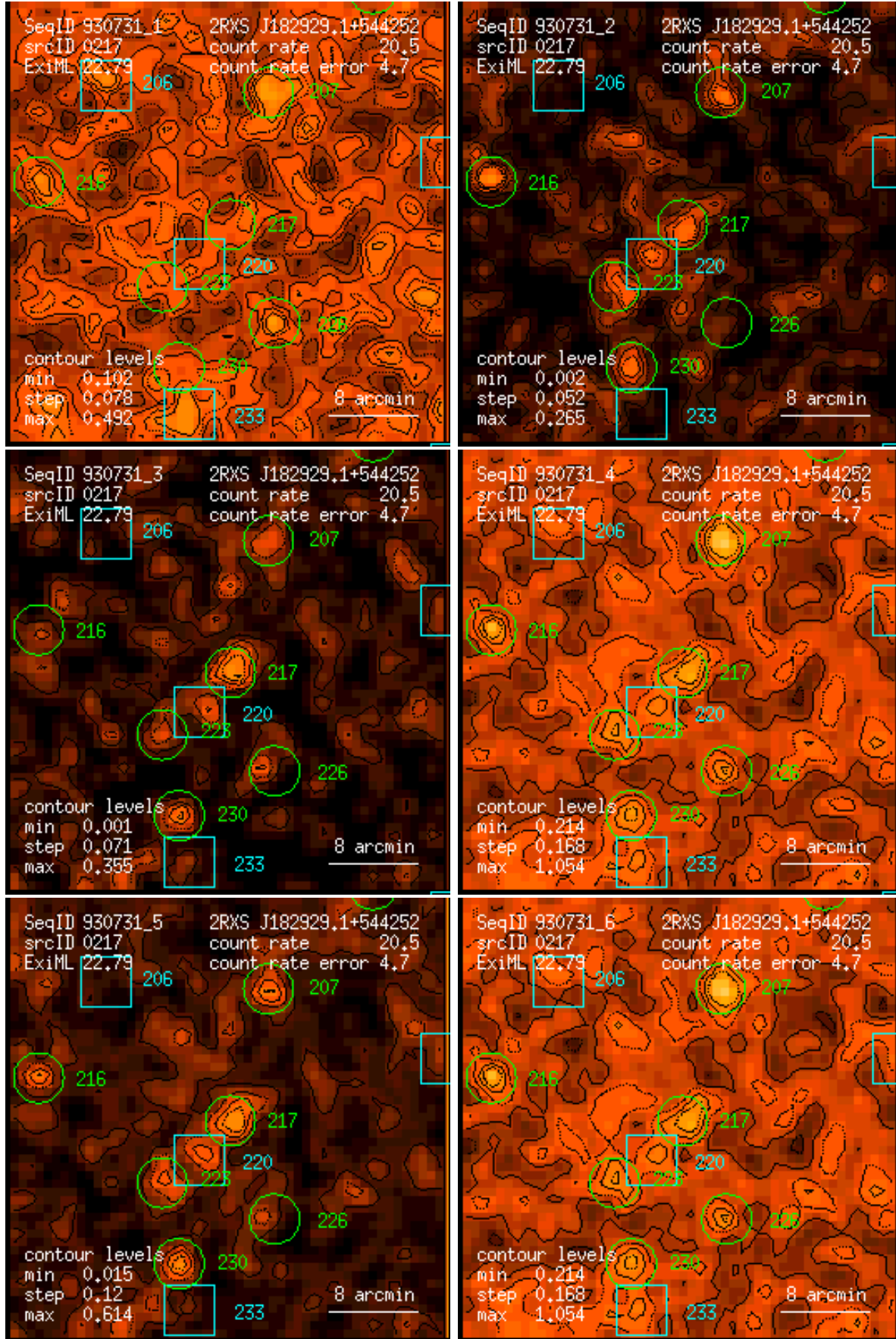
Figure 217: RASS 930731: detection 0217: band rate images, Gaussian filter: (1) PSPC channels 11 – 41, (2) 52 – 90, (3) 91 – 201, (4) 11 – 235, (5) 52 – 201, (6) 11 – 201. Broad band rates in counts/ks. Band rate contour levels in counts/ks/arcmin 2 .
