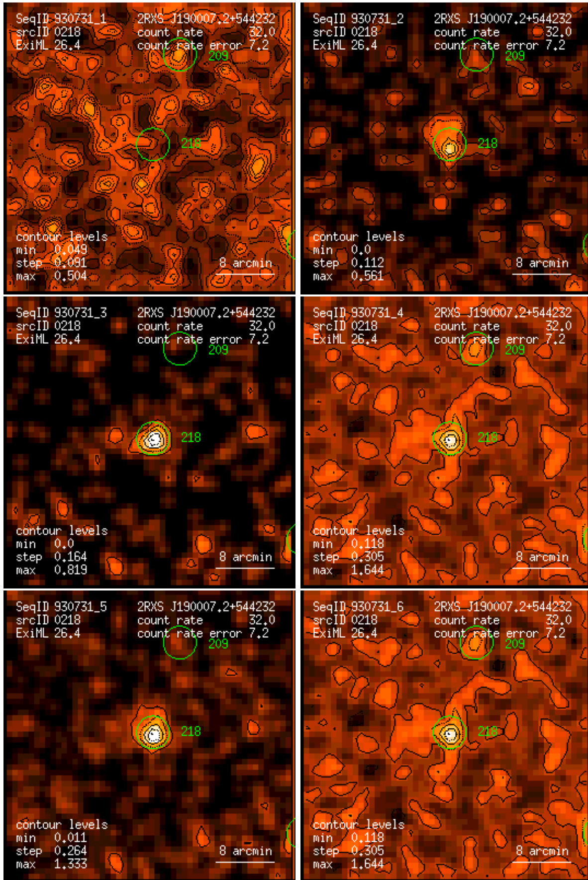
Figure 218: RASS 930731: detection 0218: band rate images, Gaussian filter: (1) PSPC channels 11 – 41, (2) 52 – 90, (3) 91 – 201, (4) 11 – 235, (5) 52 – 201, (6) 11 – 201. Broad band rates in counts/ks. Band rate contour levels in counts/ks/arcmin 2 .
