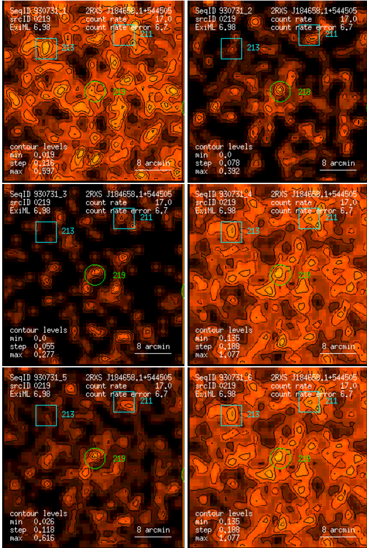
Figure 219: RASS 930731: detection 0219: band rate images, Gaussian filter: (1) PSPC channels 11 – 41, (2) 52 – 90, (3) 91 – 201, (4) 11 – 235, (5) 52 – 201, (6) 11 – 201. Broad band rates in counts/ks. Band rate contour levels in counts/ks/arcmin 2 .
