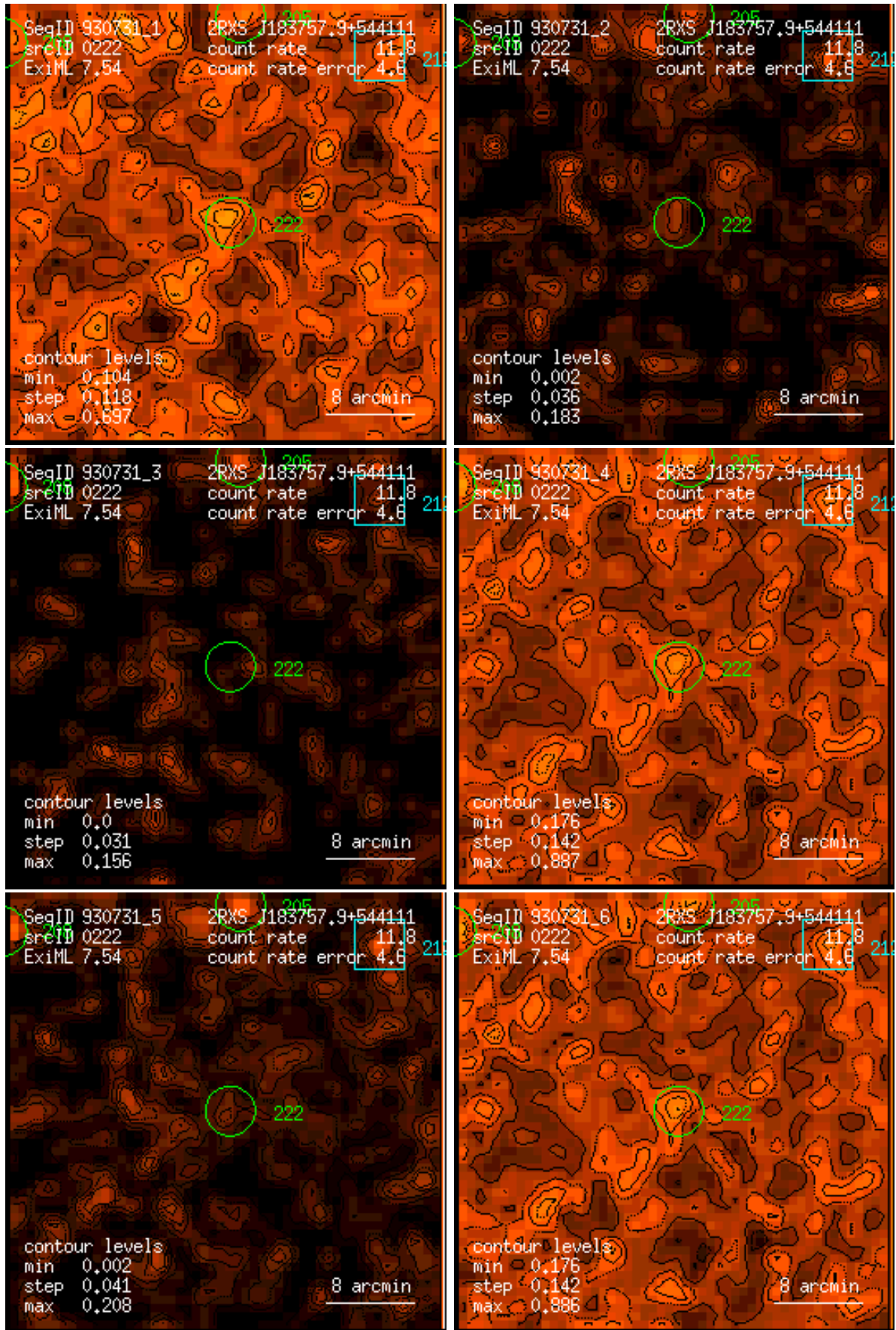
Figure 222: RASS 930731: detection 0222: band rate images, Gaussian filter: (1) PSPC channels 11 – 41, (2) 52 – 90, (3) 91 – 201, (4) 11 – 235, (5) 52 – 201, (6) 11 – 201. Broad band rates in counts/ks. Band rate contour levels in counts/ks/arcmin 2 .
