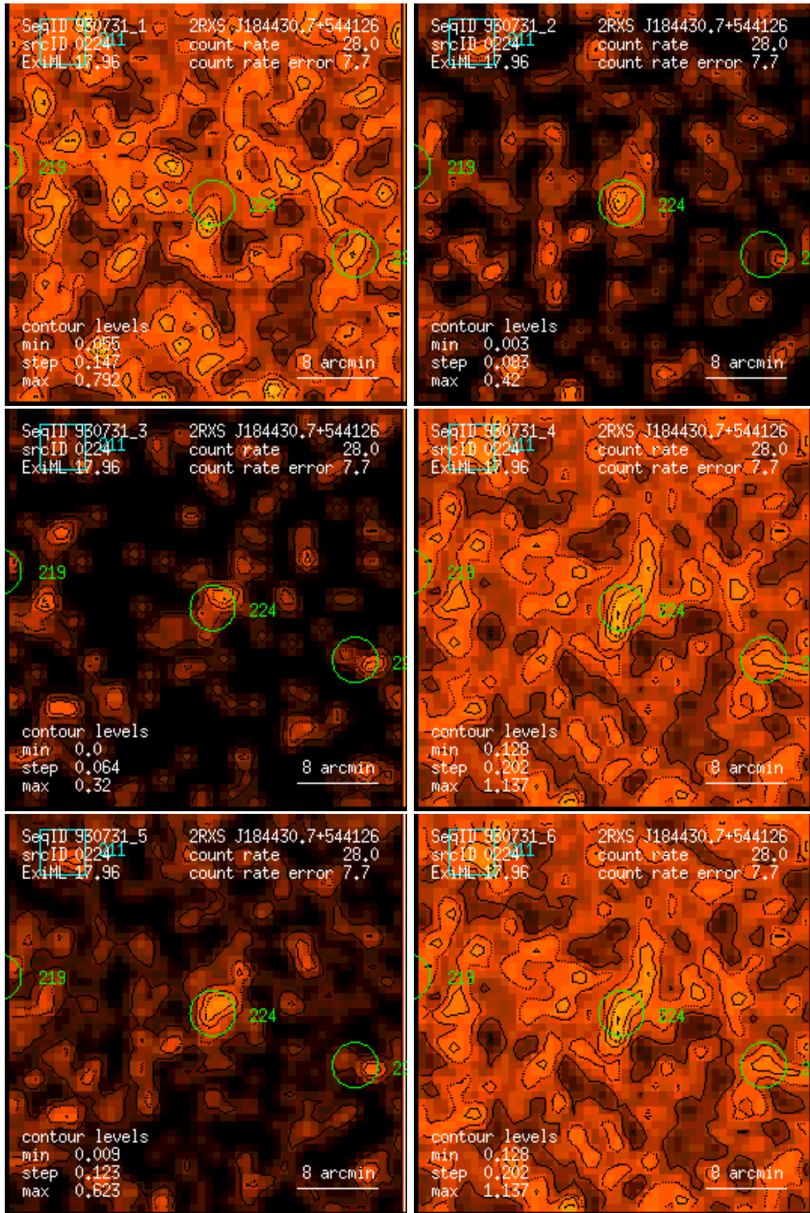
Figure 224: RASS 930731: detection 0224: band rate images, Gaussian filter: (1) PSPC channels 11 – 41, (2) 52 – 90, (3) 91 – 201, (4) 11 – 235, (5) 52 – 201, (6) 11 – 201. Broad band rates in counts/ks. Band rate contour levels in counts/ks/arcmin 2 .
