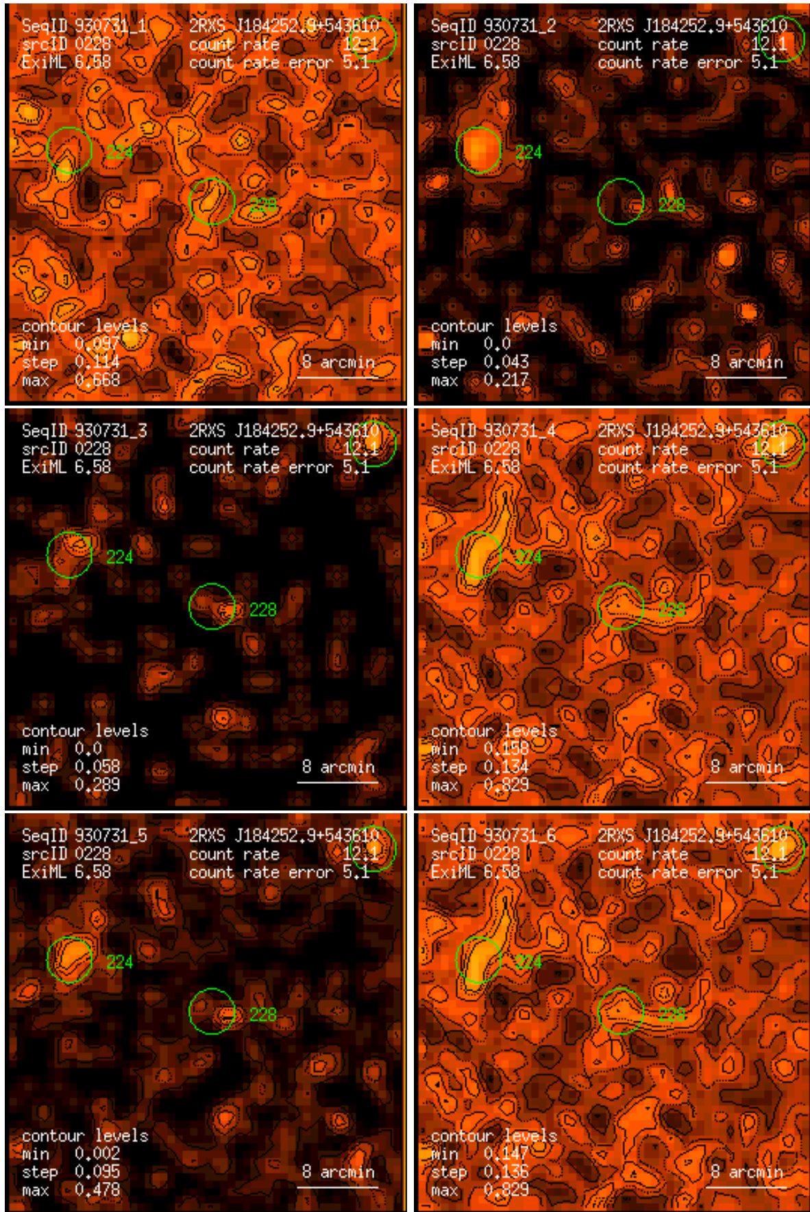
Figure 228: RASS 930731: detection 0228: band rate images, Gaussian filter: (1) PSPC channels 11 – 41, (2) 52 – 90, (3) 91 – 201, (4) 11 – 235, (5) 52 – 201, (6) 11 – 201. Broad band rates in counts/ks. Band rate contour levels in counts/ks/arcmin 2 .
