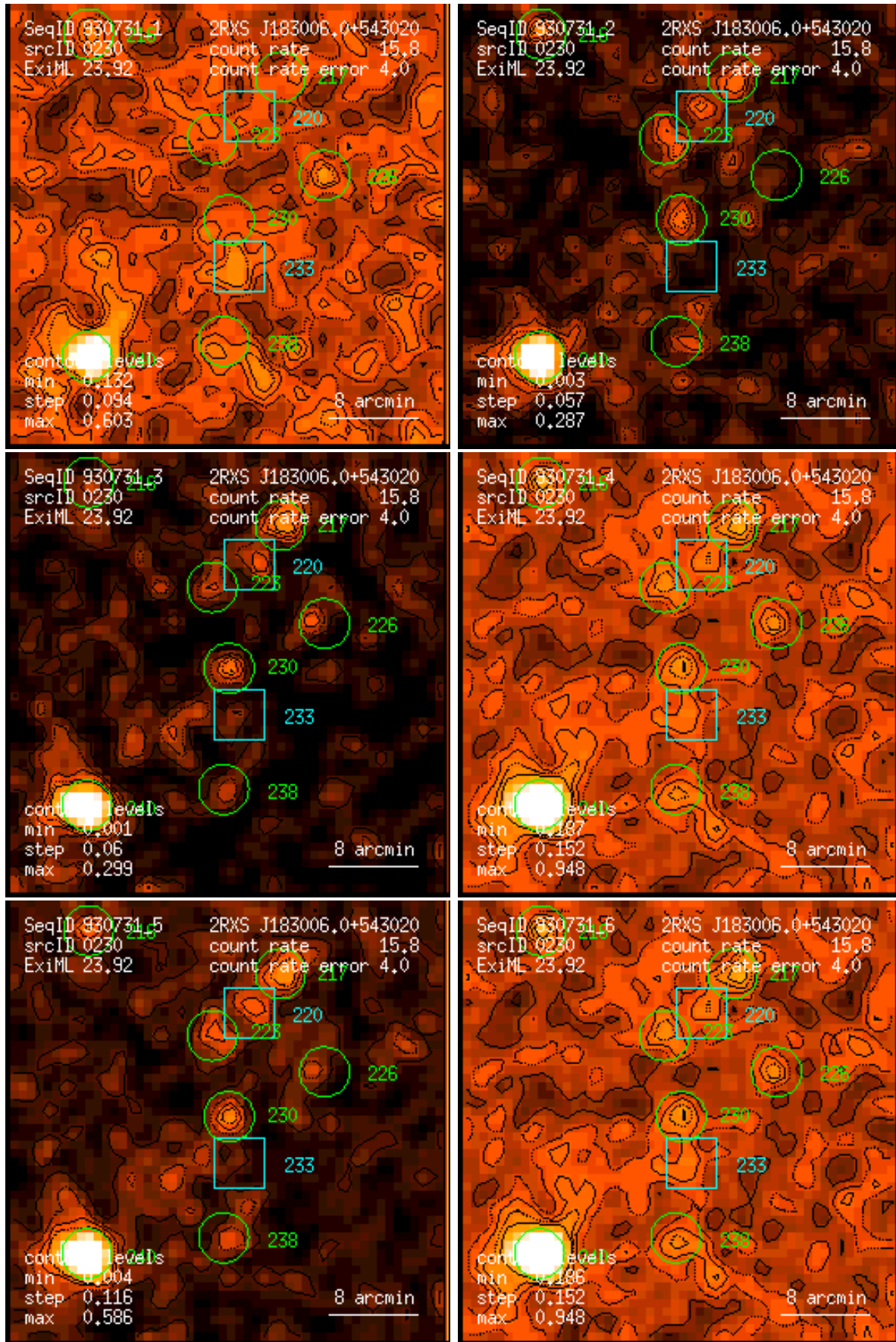
Figure 230: RASS 930731: detection 0230: band rate images, Gaussian filter: (1) PSPC channels 11 – 41, (2) 52 – 90, (3) 91 – 201, (4) 11 – 235, (5) 52 – 201, (6) 11 – 201. Broad band rates in counts/ks. Band rate contour levels in counts/ks/arcmin 2 .
