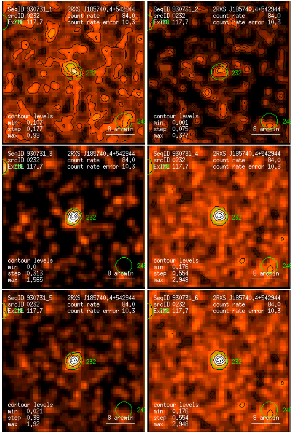
Figure 232: RASS 930731: detection 0232: band rate images, Gaussian filter: (1) PSPC channels 11 – 41, (2) 52 – 90, (3) 91 – 201, (4) 11 – 235, (5) 52 – 201, (6) 11 – 201. Broad band rates in counts/ks. Band rate contour levels in counts/ks/arcmin 2 .
