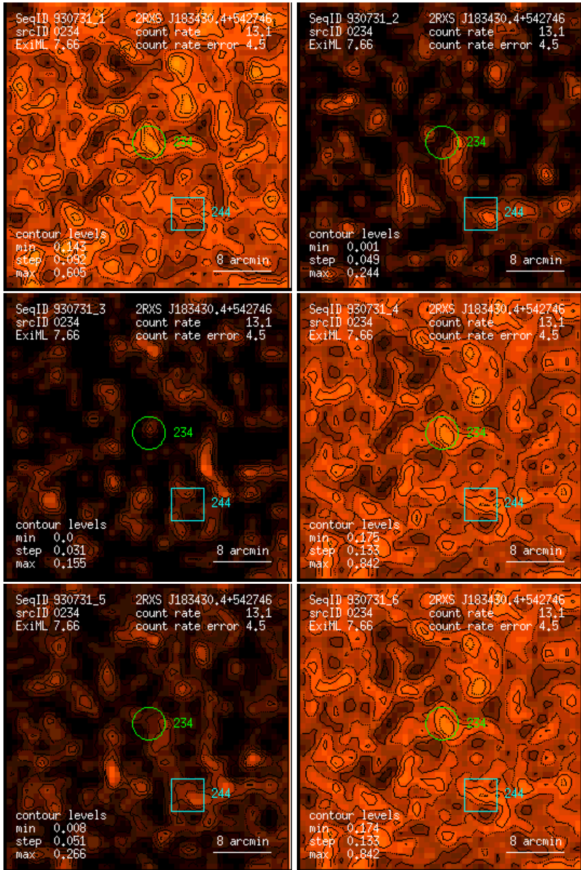
Figure 234: RASS 930731: detection 0234: band rate images, Gaussian filter: (1) PSPC channels 11 – 41, (2) 52 – 90, (3) 91 – 201, (4) 11 – 235, (5) 52 – 201, (6) 11 – 201. Broad band rates in counts/ks. Band rate contour levels in counts/ks/arcmin 2 .
