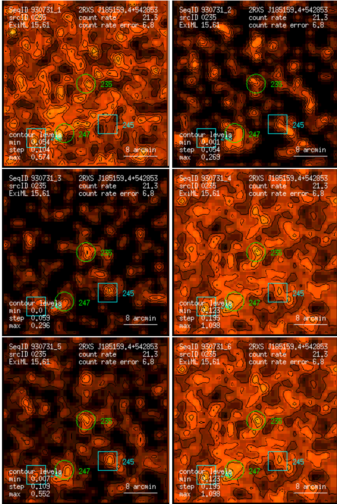
Figure 235: RASS 930731: detection 0235: band rate images, Gaussian filter: (1) PSPC channels 11 – 41, (2) 52 – 90, (3) 91 – 201, (4) 11 – 235, (5) 52 – 201, (6) 11 – 201. Broad band rates in counts/ks. Band rate contour levels in counts/ks/arcmin 2 .
