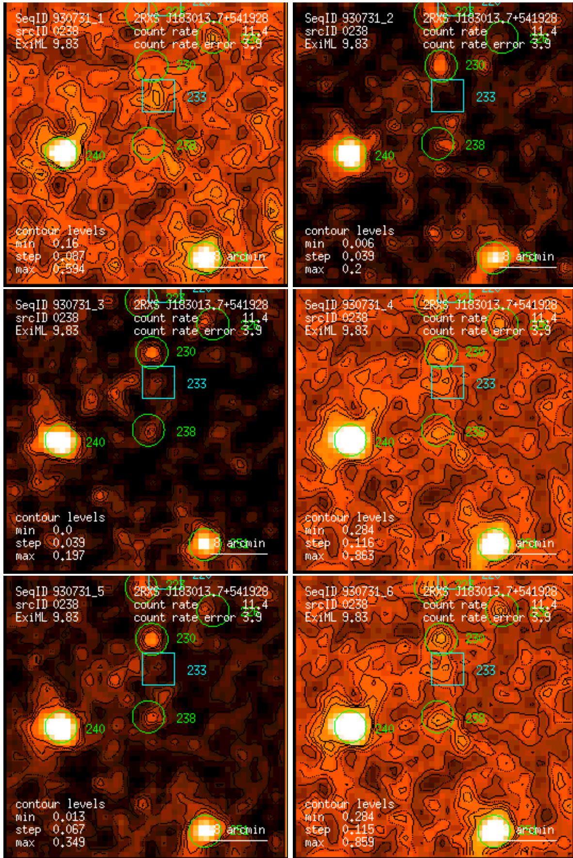
Figure 238: RASS 930731: detection 0238: band rate images, Gaussian filter: (1) PSPC channels 11 – 41, (2) 52 – 90, (3) 91 – 201, (4) 11 – 235, (5) 52 – 201, (6) 11 – 201. Broad band rates in counts/ks. Band rate contour levels in counts/ks/arcmin 2 .
