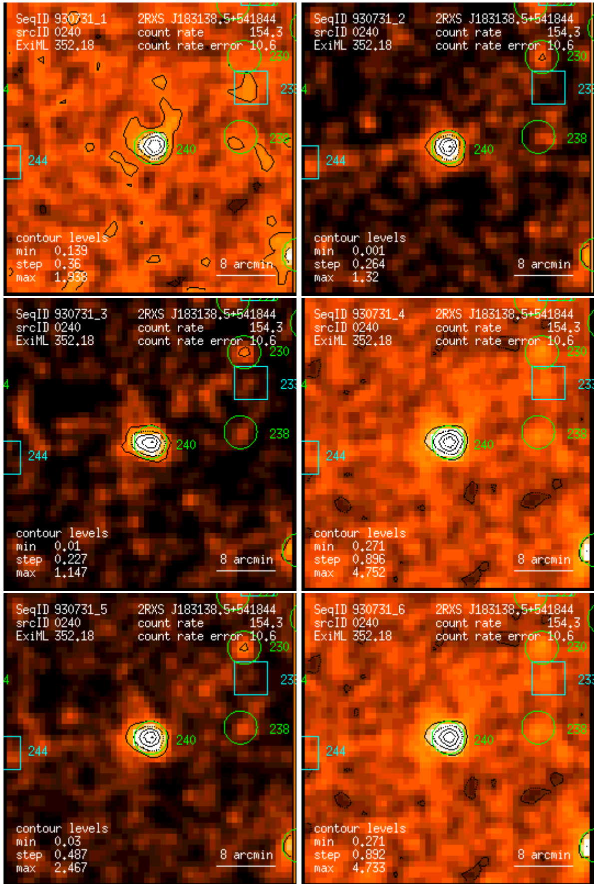
Figure 240: RASS 930731: detection 0240: band rate images, Gaussian filter: (1) PSPC channels 11 – 41, (2) 52 – 90, (3) 91 – 201, (4) 11 – 235, (5) 52 – 201, (6) 11 – 201. Broad band rates in counts/ks. Band rate contour levels in counts/ks/arcmin 2 .
