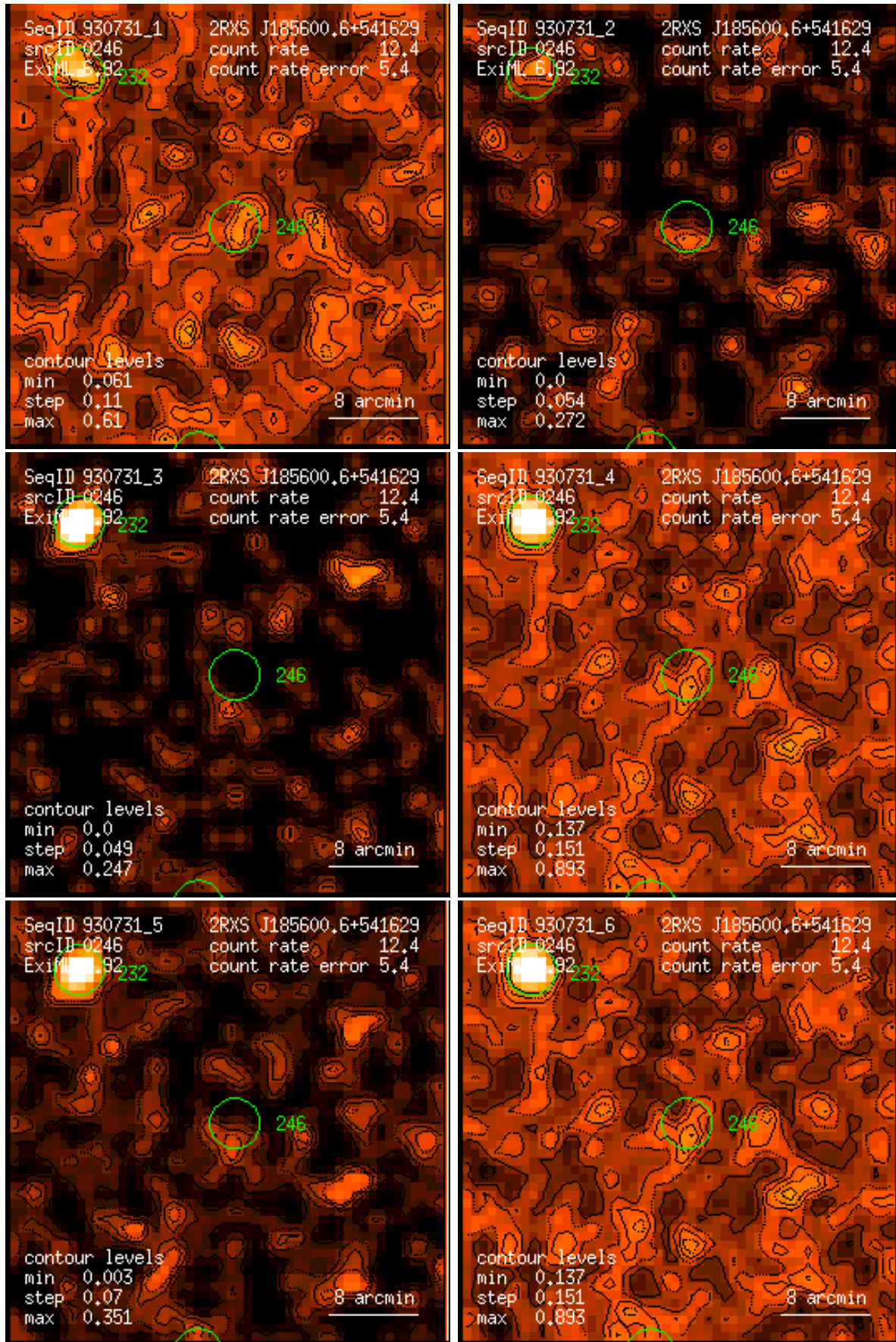
Figure 246: RASS 930731: detection 0246: band rate images, Gaussian filter: (1) PSPC channels 11 – 41, (2) 52 – 90, (3) 91 – 201, (4) 11 – 235, (5) 52 – 201, (6) 11 – 201. Broad band rates in counts/ks. Band rate contour levels in counts/ks/arcmin 2 .
