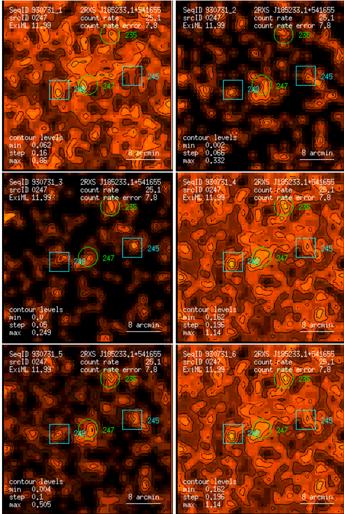
Figure 247: RASS 930731: detection 0247: band rate images, Gaussian filter: (1) PSPC channels 11 – 41, (2) 52 – 90, (3) 91 – 201, (4) 11 – 235, (5) 52 – 201, (6) 11 – 201. Broad band rates in counts/ks. Band rate contour levels in counts/ks/arcmin 2 .
