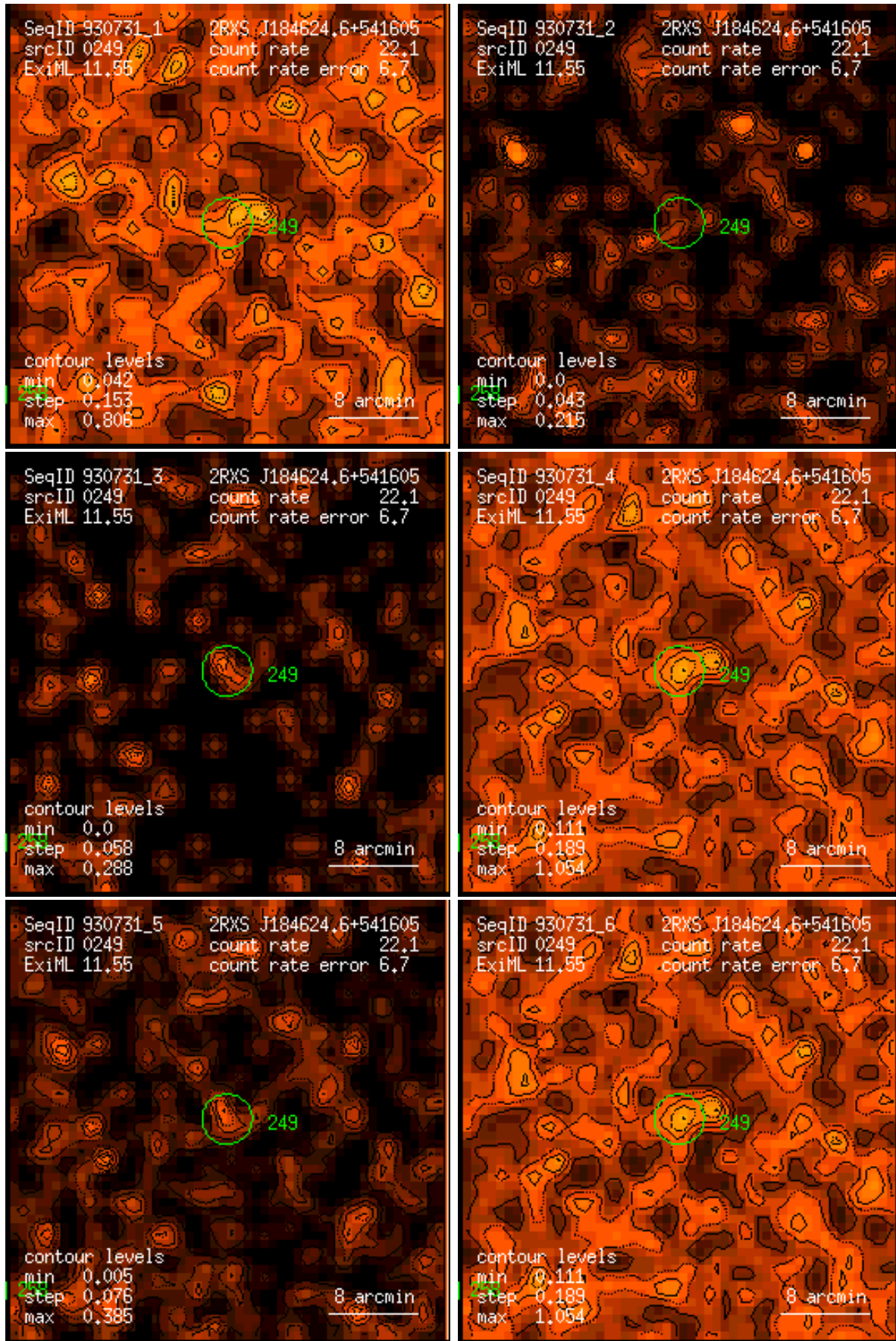
Figure 249: RASS 930731: detection 0249: band rate images, Gaussian filter: (1) PSPC channels 11 – 41, (2) 52 – 90, (3) 91 – 201, (4) 11 – 235, (5) 52 – 201, (6) 11 – 201. Broad band rates in counts/ks. Band rate contour levels in counts/ks/arcmin 2 .
