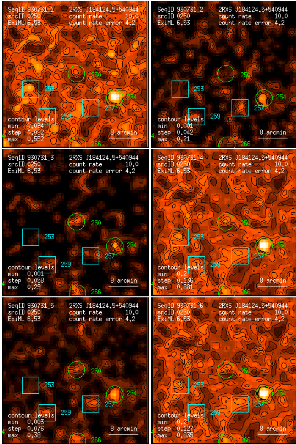
Figure 250: RASS 930731: detection 0250: band rate images, Gaussian filter: (1) PSPC channels 11 – 41, (2) 52 – 90, (3) 91 – 201, (4) 11 – 235, (5) 52 – 201, (6) 11 – 201. Broad band rates in counts/ks. Band rate contour levels in counts/ks/arcmin 2 .
