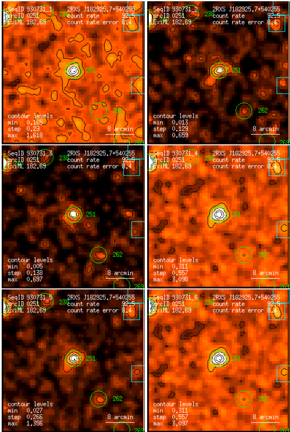
Figure 251: RASS 930731: detection 0251: band rate images, Gaussian filter: (1) PSPC channels 11 – 41, (2) 52 – 90, (3) 91 – 201, (4) 11 – 235, (5) 52 – 201, (6) 11 – 201. Broad band rates in counts/ks. Band rate contour levels in counts/ks/arcmin 2 .
