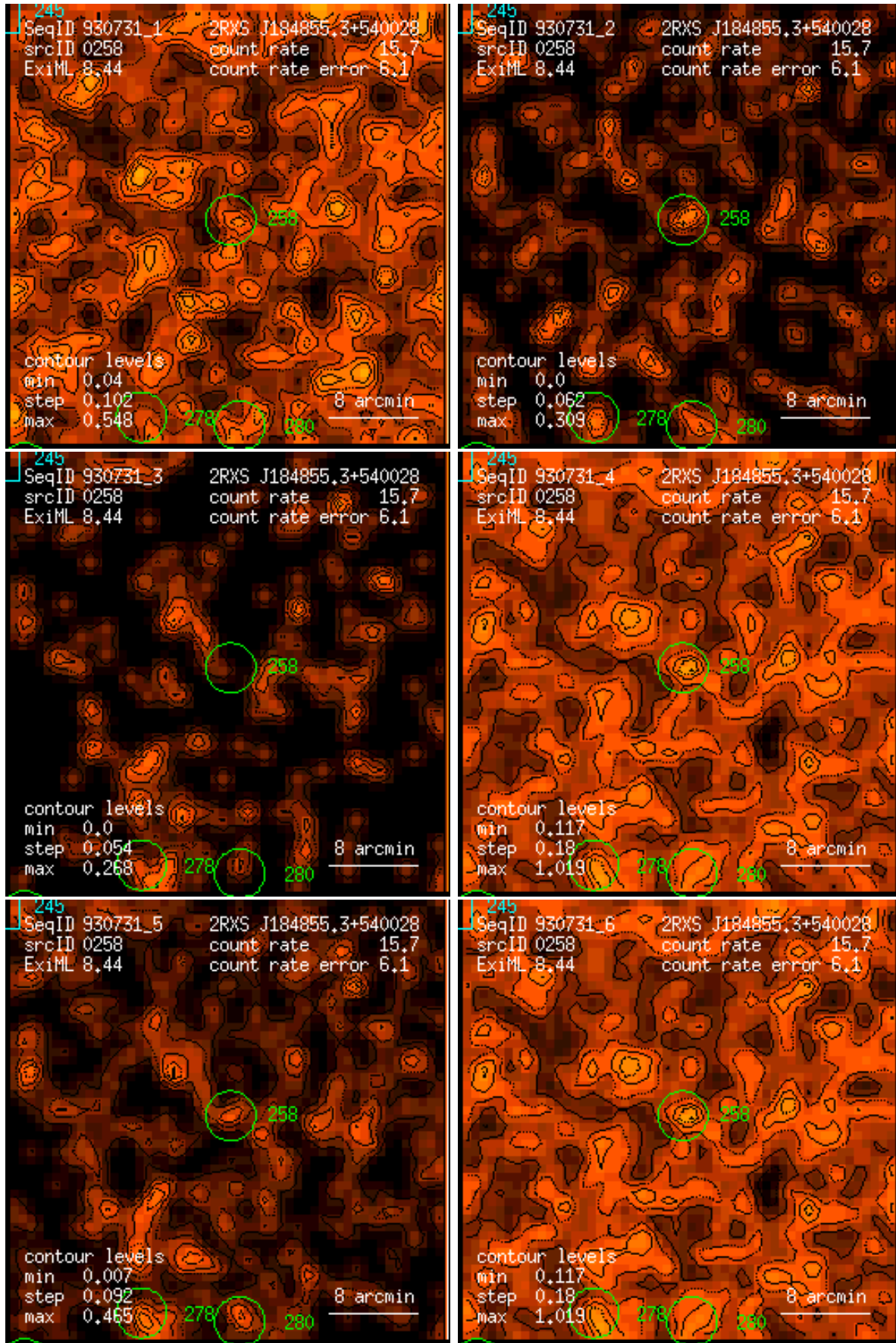
Figure 258: RASS 930731: detection 0258: band rate images, Gaussian filter: (1) PSPC channels 11 – 41, (2) 52 – 90, (3) 91 – 201, (4) 11 – 235, (5) 52 – 201, (6) 11 – 201. Broad band rates in counts/ks. Band rate contour levels in counts/ks/arcmin 2 .
