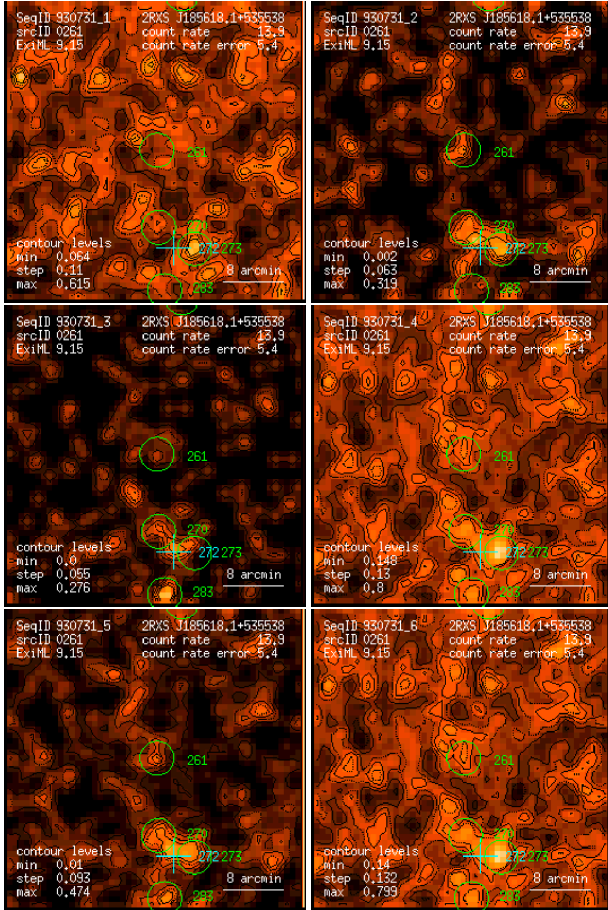
Figure 261: RASS 930731: detection 0261: band rate images, Gaussian filter: (1) PSPC channels 11 – 41, (2) 52 – 90, (3) 91 – 201, (4) 11 – 235, (5) 52 – 201, (6) 11 – 201. Broad band rates in counts/ks. Band rate contour levels in counts/ks/arcmin 2 .
