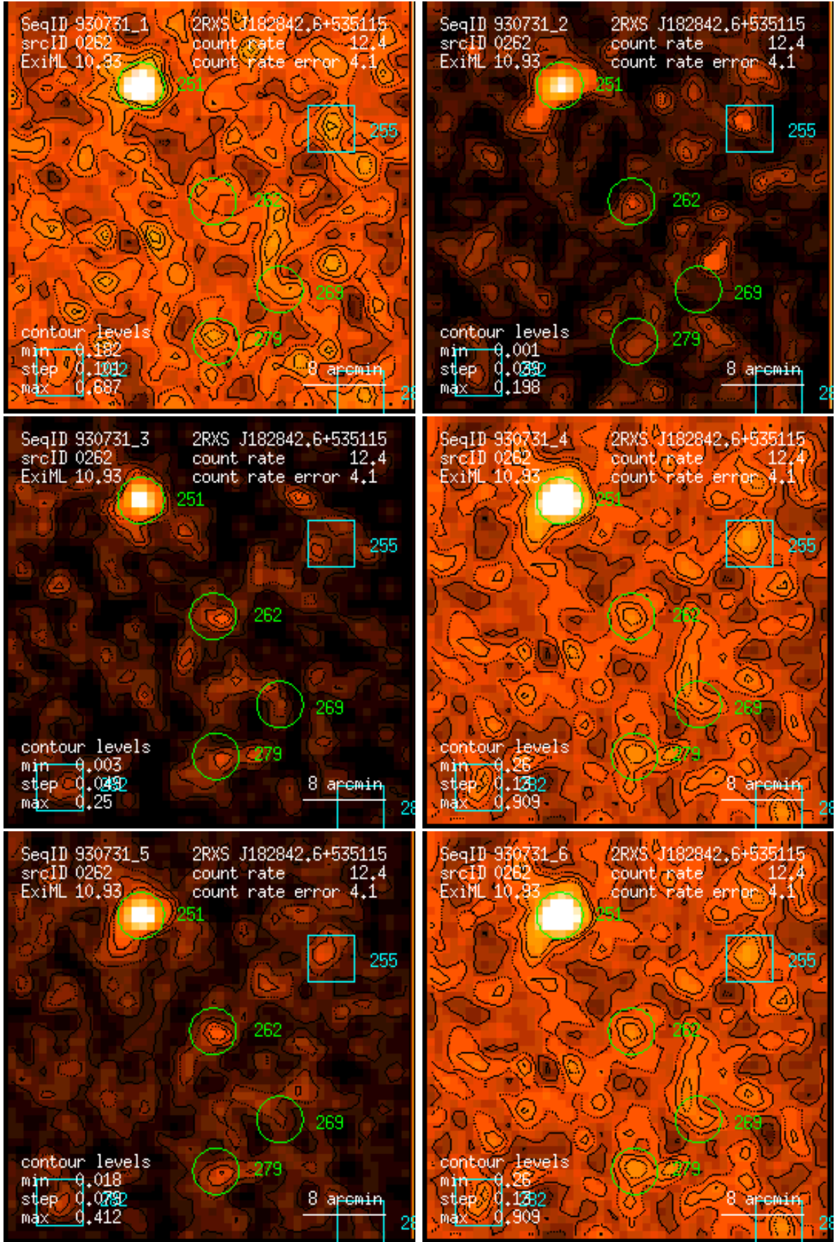
Figure 262: RASS 930731: detection 0262: band rate images, Gaussian filter: (1) PSPC channels 11 – 41, (2) 52 – 90, (3) 91 – 201, (4) 11 – 235, (5) 52 – 201, (6) 11 – 201. Broad band rates in counts/ks. Band rate contour levels in counts/ks/arcmin 2 .
