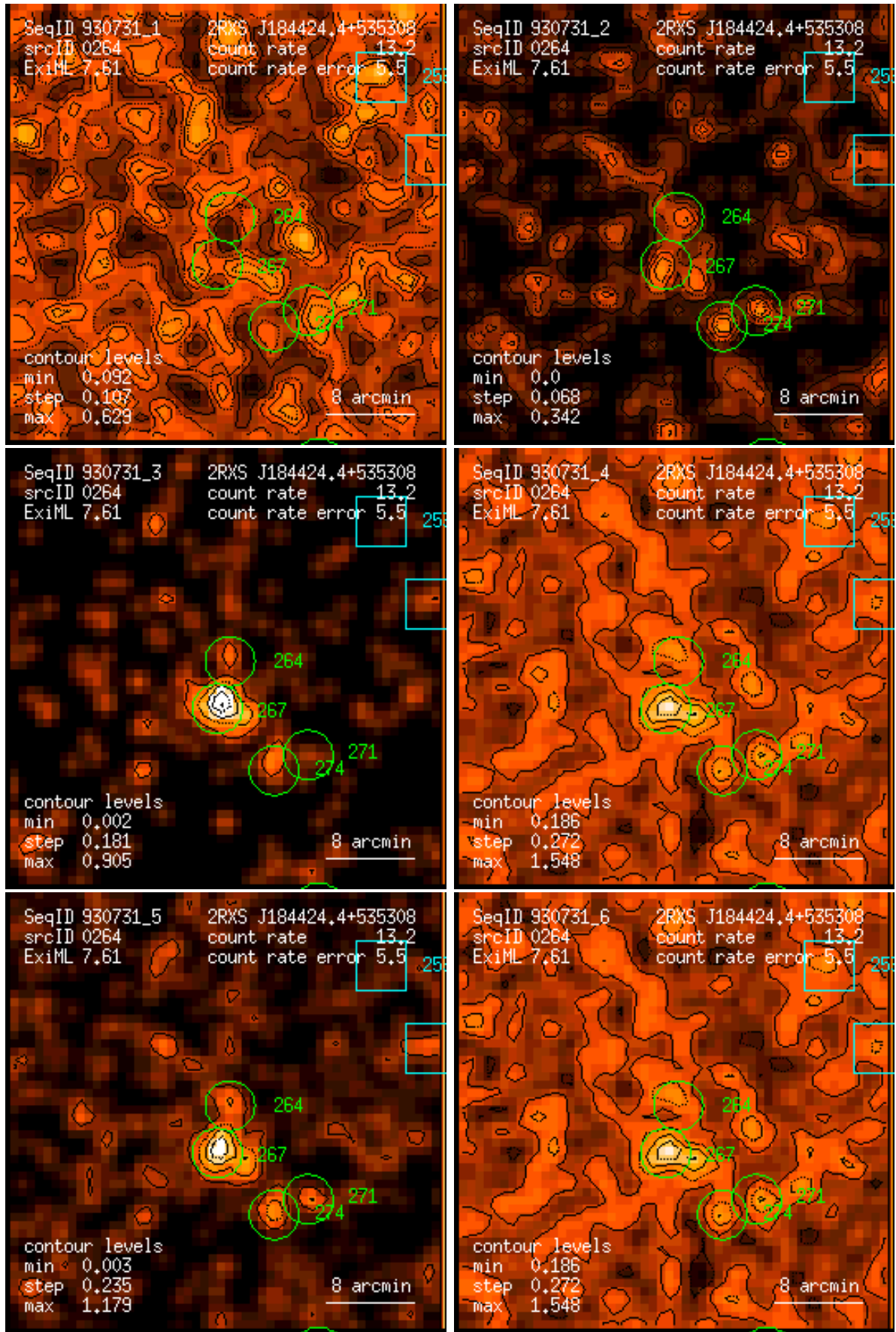
Figure 264: RASS 930731: detection 0264: band rate images, Gaussian filter: (1) PSPC channels 11 – 41, (2) 52 – 90, (3) 91 – 201, (4) 11 – 235, (5) 52 – 201, (6) 11 – 201. Broad band rates in counts/ks. Band rate contour levels in counts/ks/arcmin 2 .
